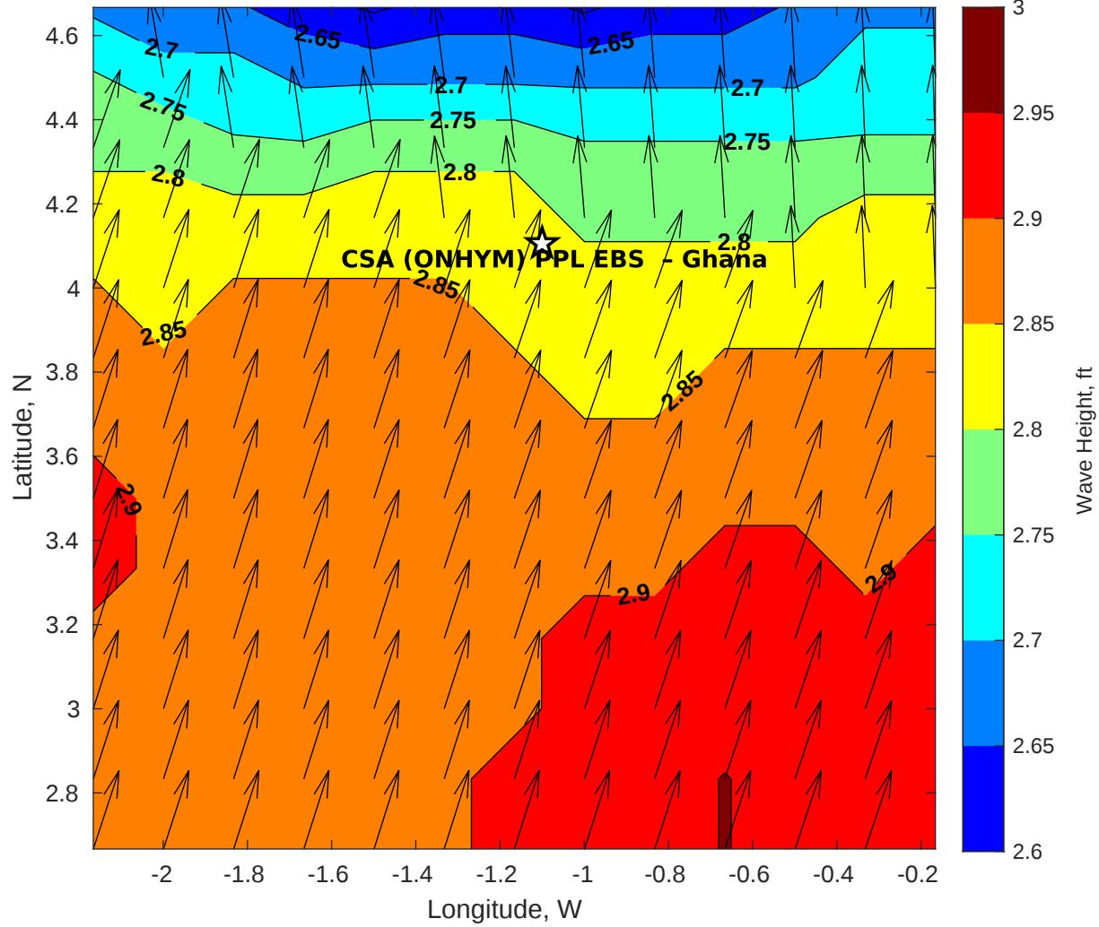
GFS Wave Height (ft) for CSA (ONHYM) PPL EBS - Ghana at 03-Jan-2026 09:00:00
