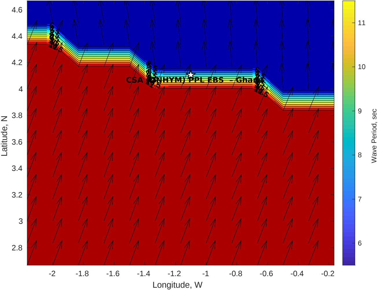
GFS Wave Period (sec) for CSA (ONHYM) PPL EBS - Ghana at 03-Jan-2026 09:00:00
