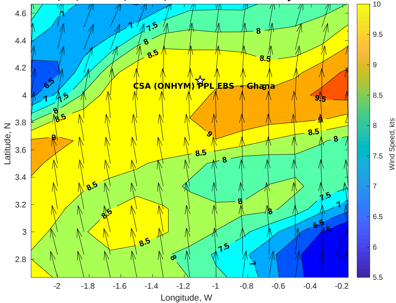
GFS Winds (kts) for CSA (ONHYM) PPL EBS - Ghana at 03-Jan-2026 09:00:00
