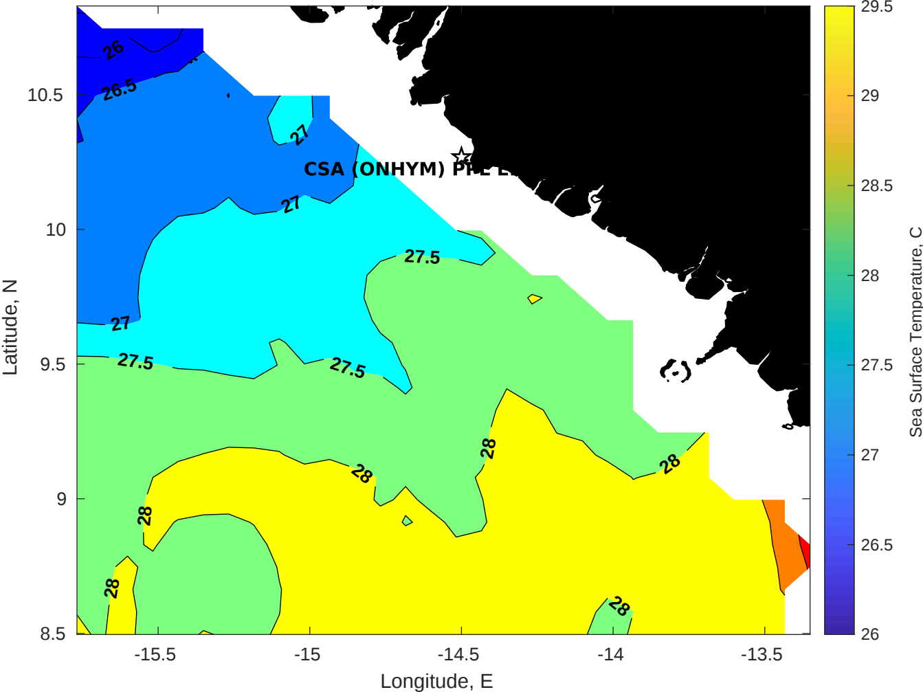
SST for CSA (ONHYM) PPL EBS - Guinea at 02-Jan-2026 00:00:00
