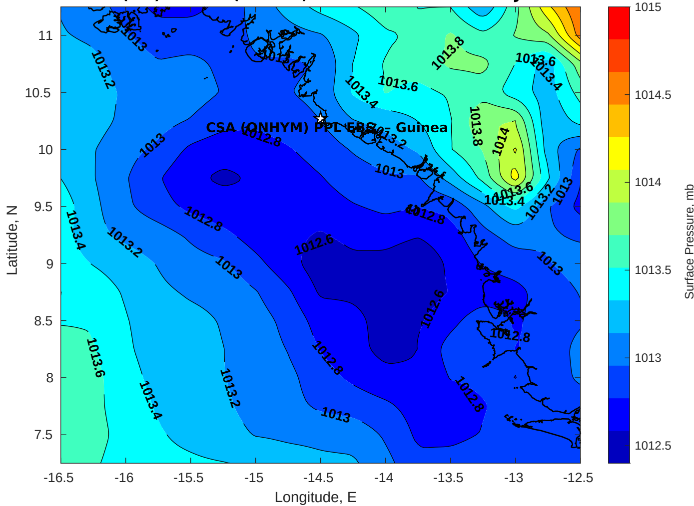
Surface Pressure (mb) for CSA (ONHYM) PPL EBS - Guinea at 04-Jan-2026 00:00:00
