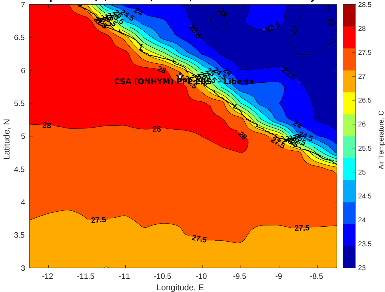
Air Temperature (C) for CSA (ONHYM) PPL EBS - Liberia at 03-Jan-2026
