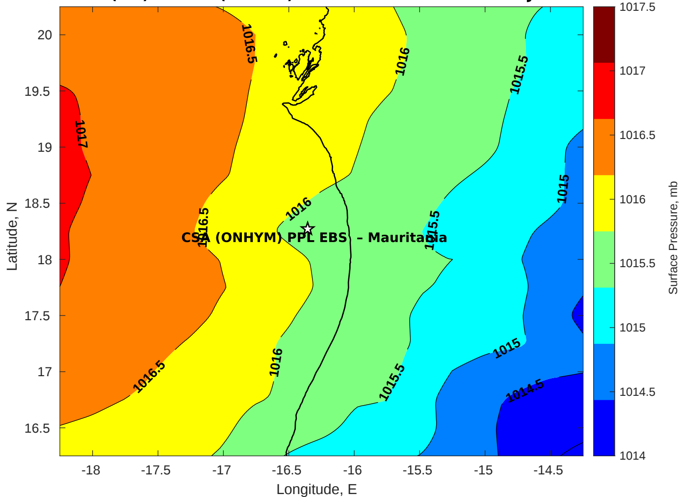
Surface Pressure (mb) for CSA (ONHYM) PPL EBS - Mauritania at 05-Jan-2026 00:00:00
