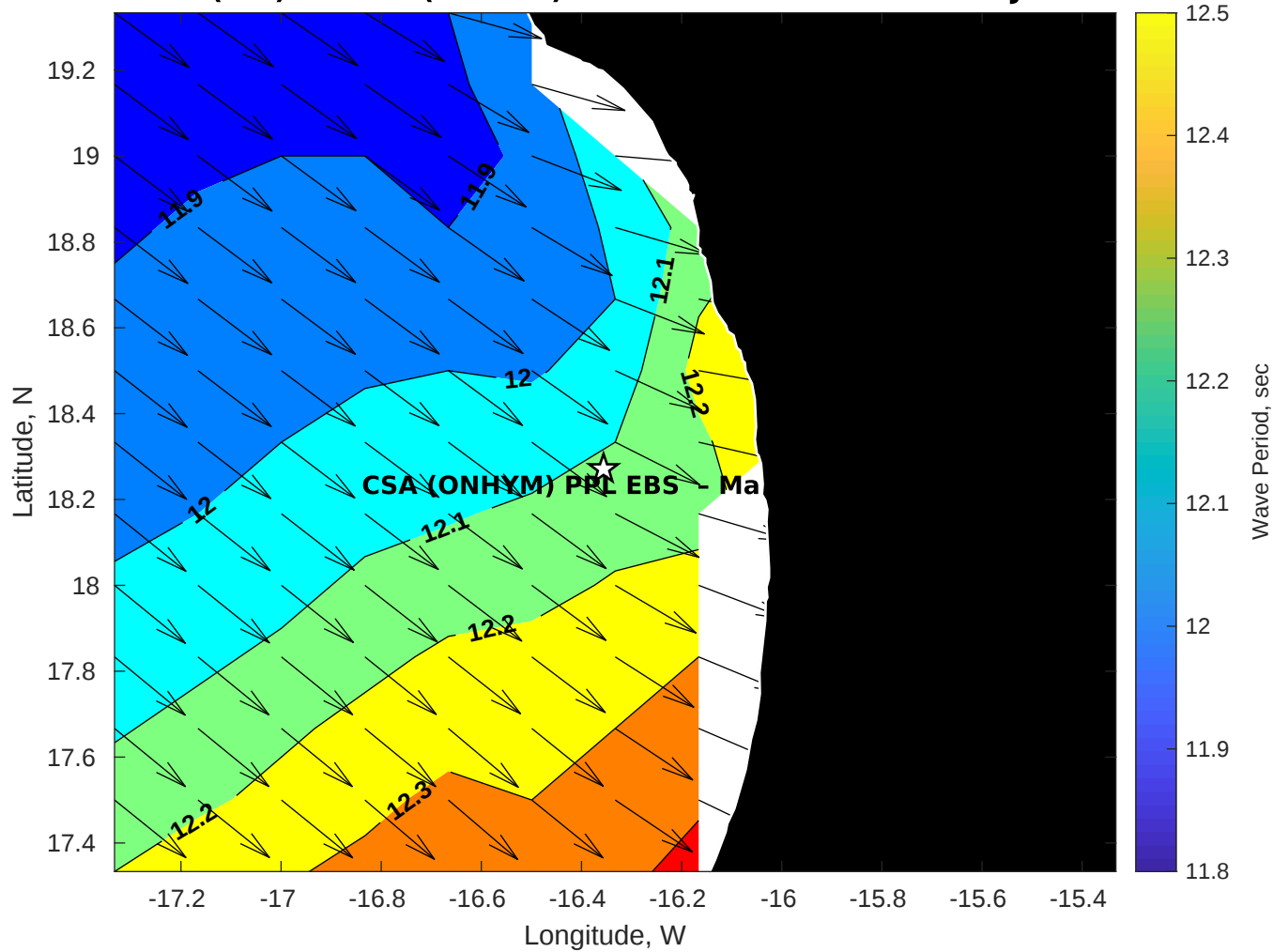
GFS Wave Period (sec) for CSA (ONHYM) PPL EBS - Mauritania at 03-Jan-2026 09:00:00
