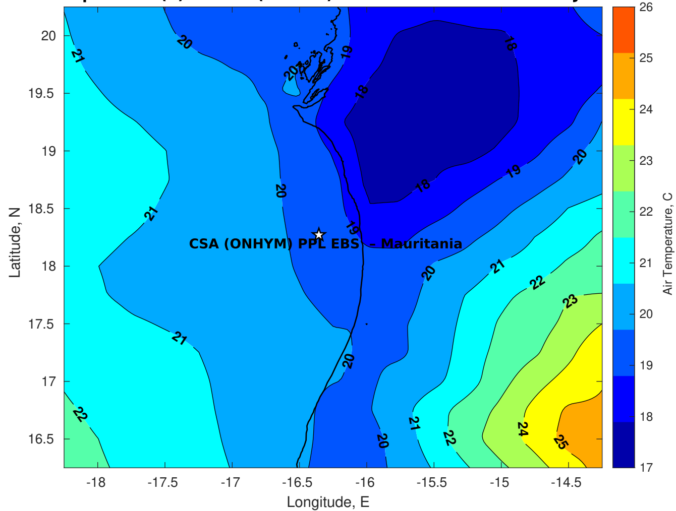
Air Temperature (C) for CSA (ONHYM) PPL EBS - Mauritania at 03-Jan-2026
