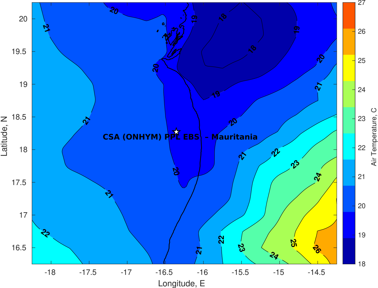
Air Temperature (C) for CSA (ONHYM) PPL EBS - Mauritania at 03-Jan-2026
