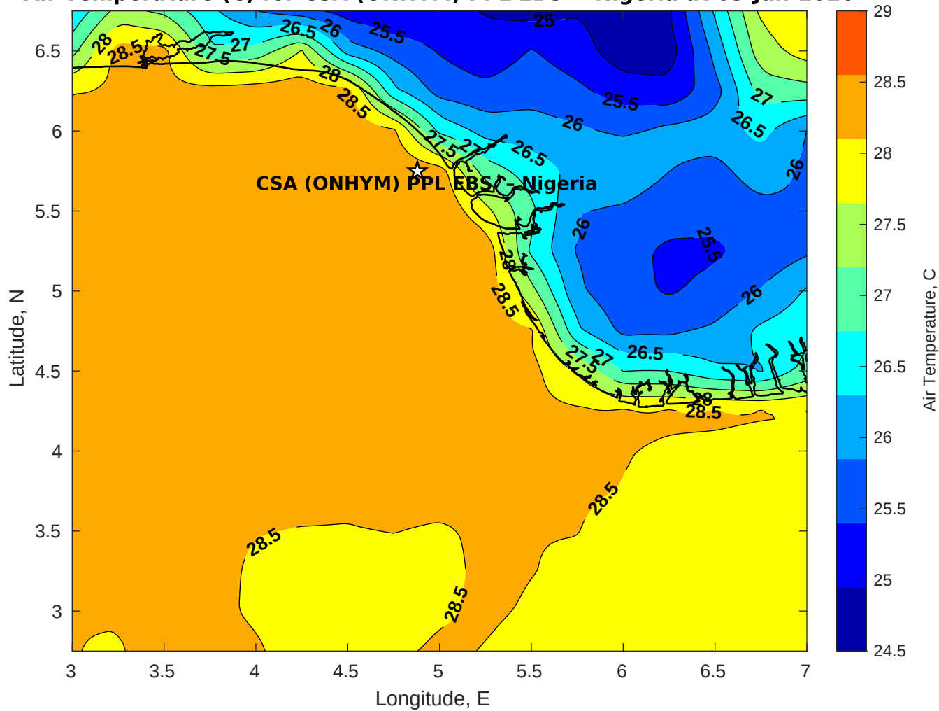
Air Temperature (C) for CSA (ONHYM) PPL EBS - Nigeria at 03-Jan-2026
