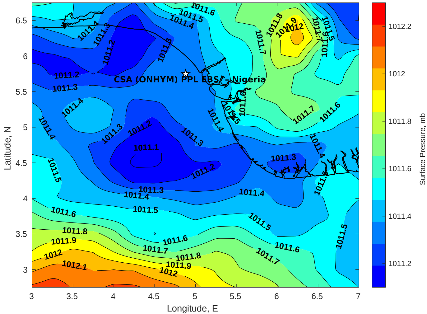
Surface Pressure (mb) for CSA (ONHYM) PPL EBS - Nigeria at 04-Jan-2026 00:00:00
