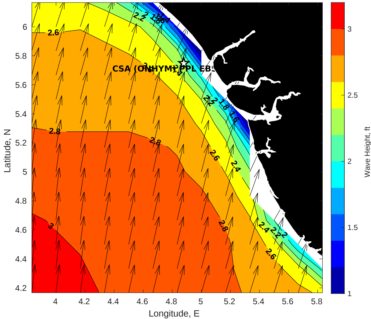
GFS Wave Height (ft) for CSA (ONHYM) PPL EBS - Nigeria at 03-Jan-2026 09:00:00
