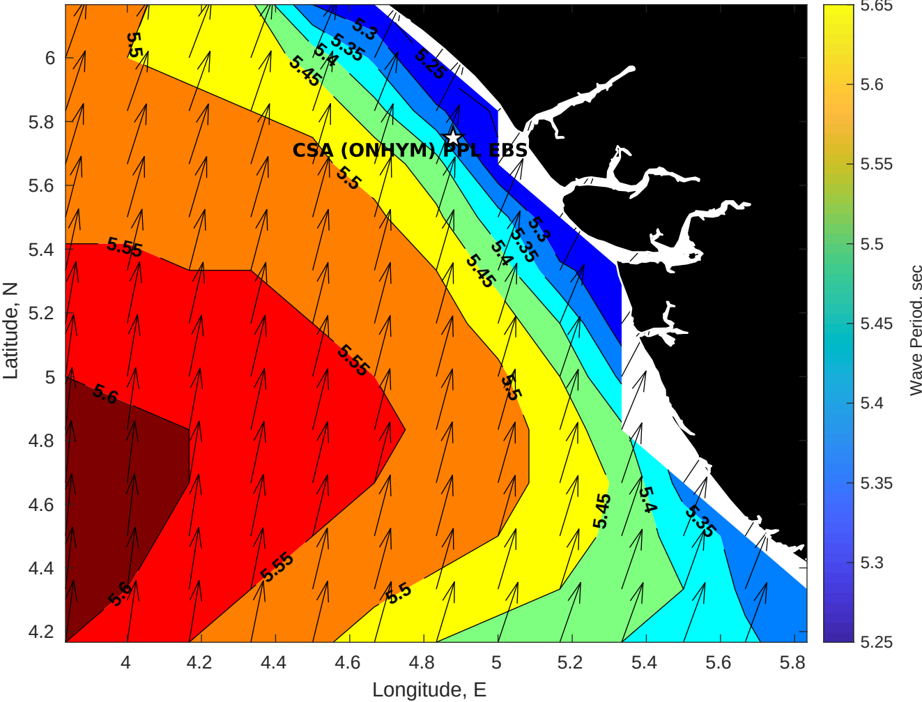
GFS Wave Period (sec) for CSA (ONHYM) PPL EBS - Nigeria at 03-Jan-2026 09:00:00
