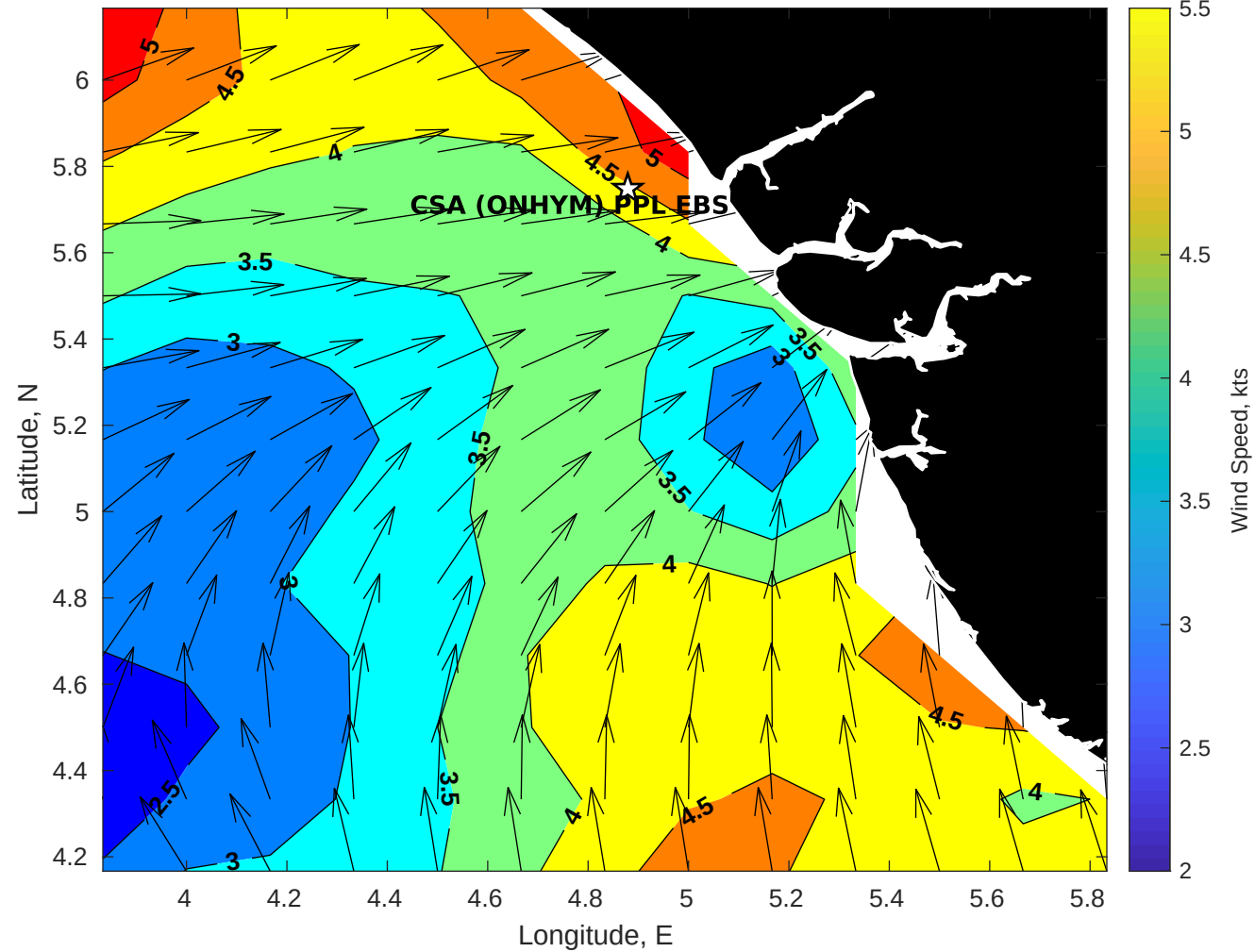
GFS Winds (kts) for CSA (ONHYM) PPL EBS - Nigeria at 03-Jan-2026 09:00:00
