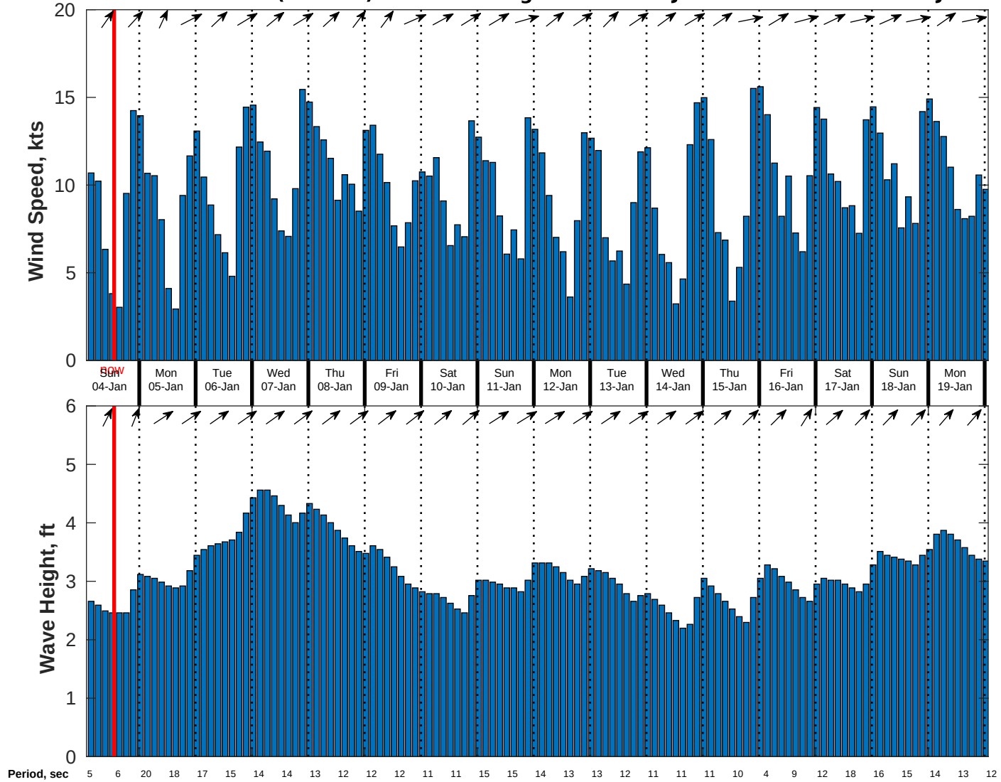
Wind & Wave Forecast for CSA (ONHYM) PPL EBS - Nigeria from 03-Jan-2026 02:00:00 to 19-Jan-2026 02:00:00
