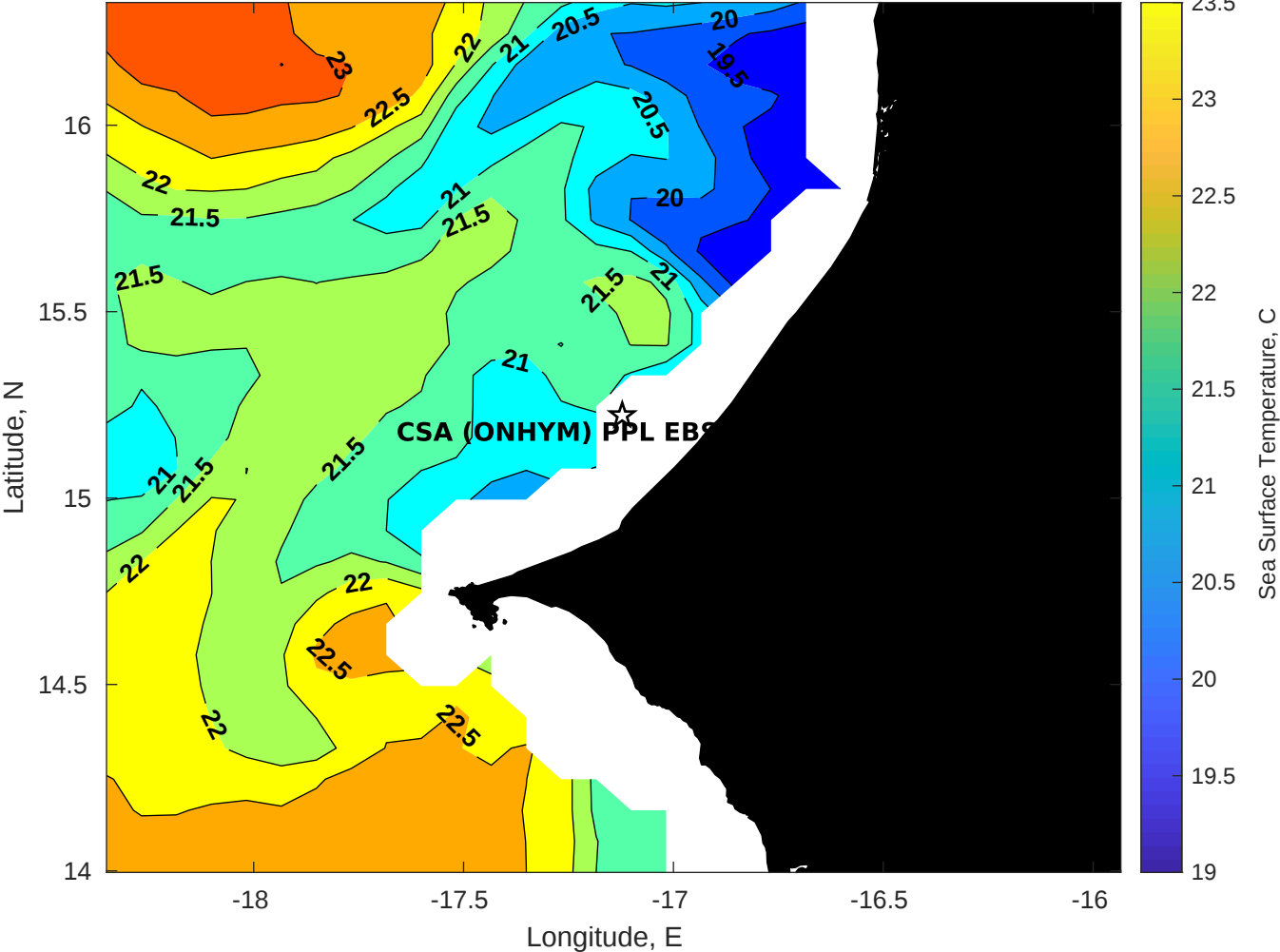
SST for CSA (ONHYM) PPL EBS - Senegal at 02-Jan-2026 00:00:00
