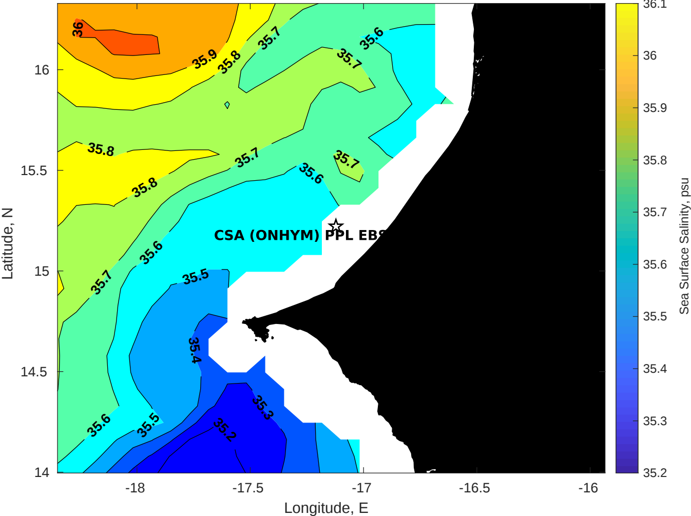
Surface Salinity for CSA (ONHYM) PPL EBS - Senegal at 02-Jan-2026 00:00:00
