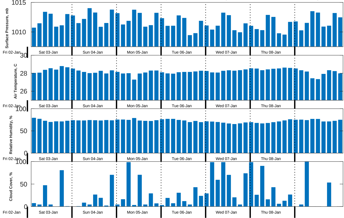
Met Forecast for CSA (ONHYM) PPL EBS - Sierra Leone from 03-Jan-2026 00:00:00 to 10-Jan-2026 00:00:00
