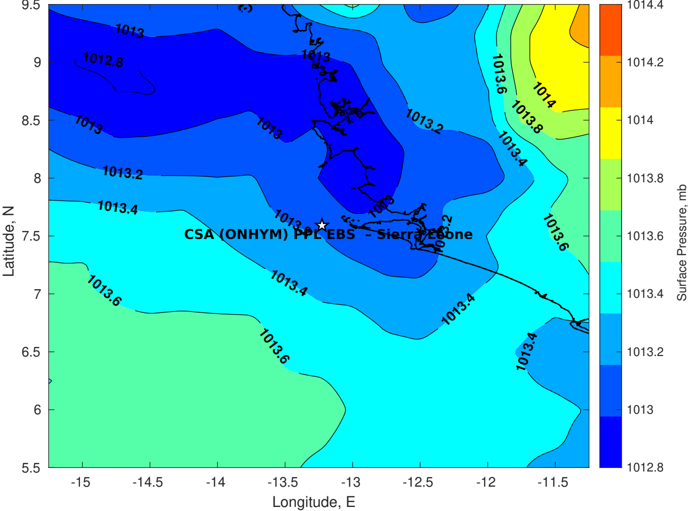
Surface Pressure (mb) for CSA (ONHYM) PPL EBS - Sierra Leone at 05-Jan-2026 00:00:00
