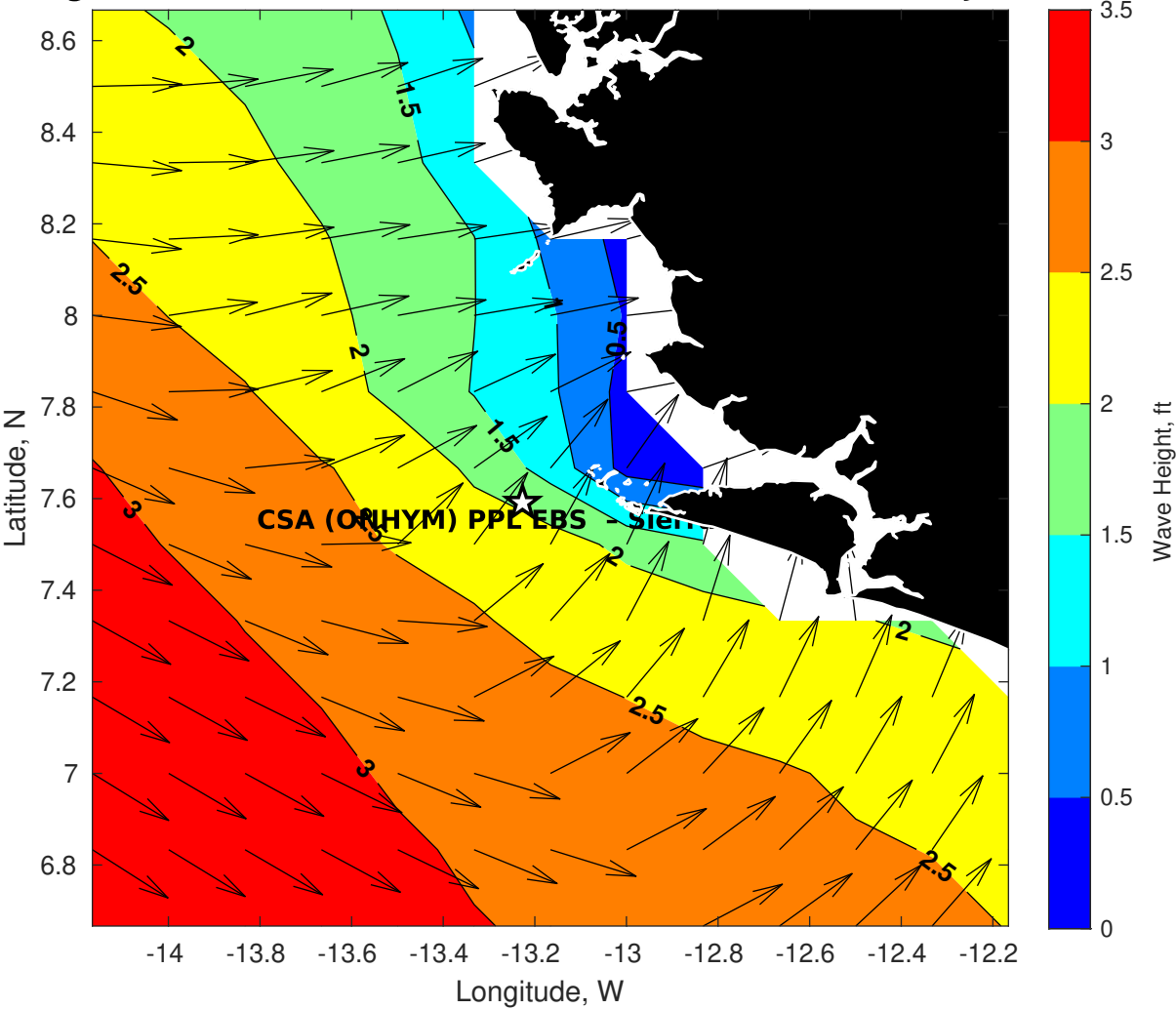
GFS Wave Height (ft) for CSA (ONHYM) PPL EBS - Sierra Leone at 03-Jan-2026 09:00:00
