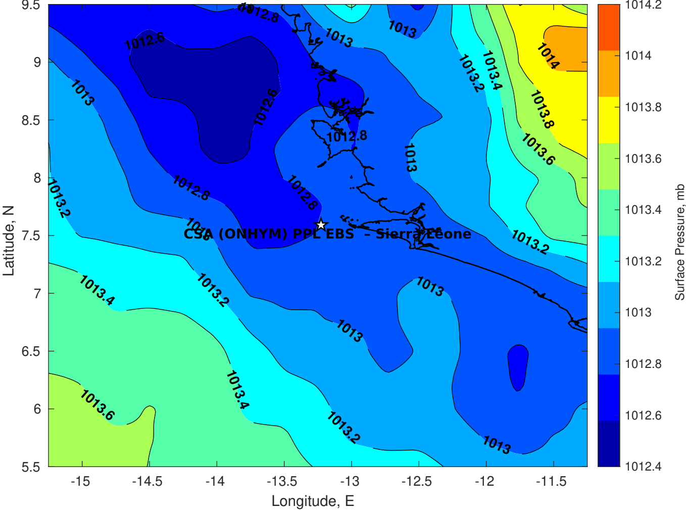
Surface Pressure (mb) for CSA (ONHYM) PPL EBS - Sierra Leone at 04-Jan-2026 00:00:00
