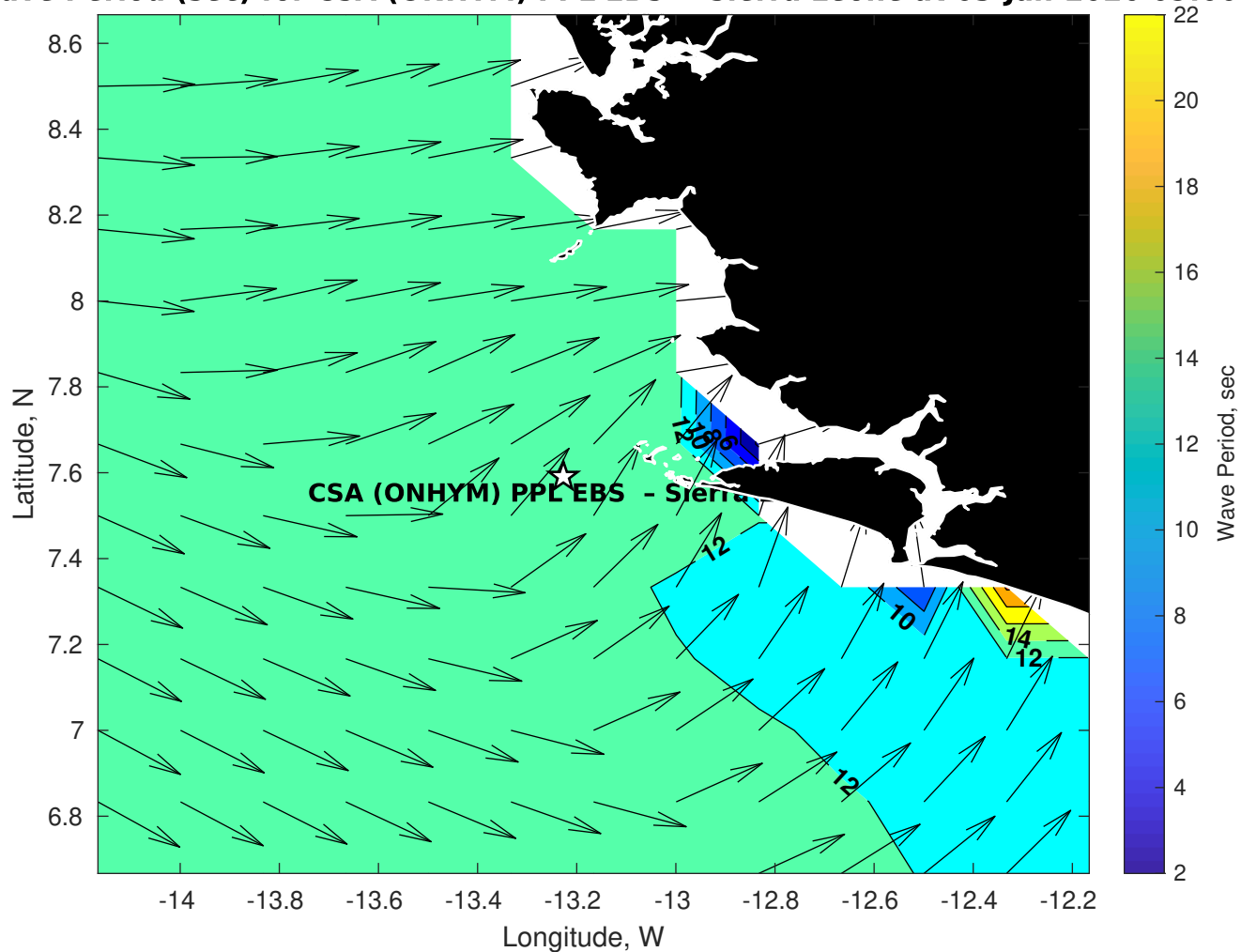
GFS Wave Period (sec) for CSA (ONHYM) PPL EBS - Sierra Leone at 03-Jan-2026 09:00:00
