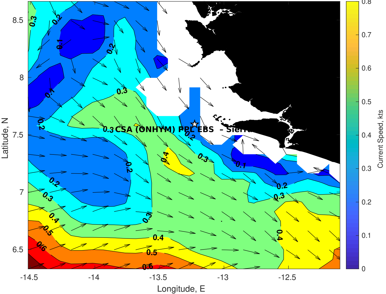
Surface Currents for CSA (ONHYM) PPL EBS - Sierra Leone at 02-Jan-2026 00:00:00
