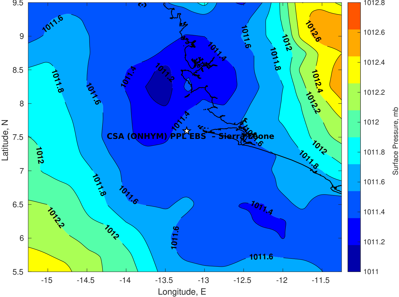
Surface Pressure (mb) for CSA (ONHYM) PPL EBS - Sierra Leone at 03-Jan-2026 00:00:00
