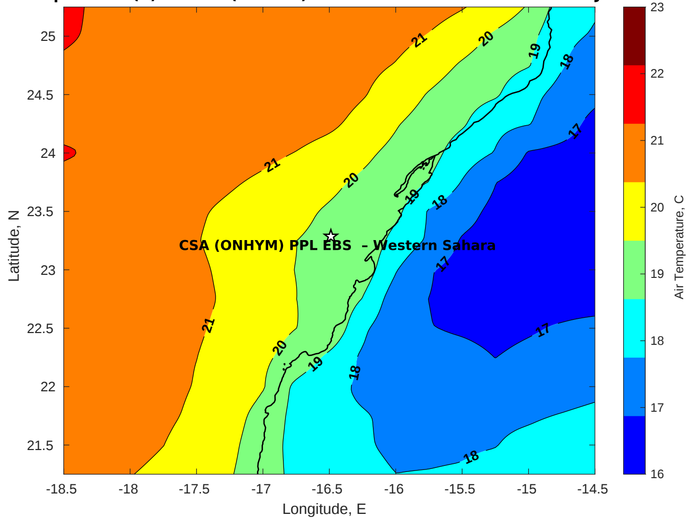
Air Temperature (C) for CSA (ONHYM) PPL EBS - Western Sahara at 03-Jan-2026
