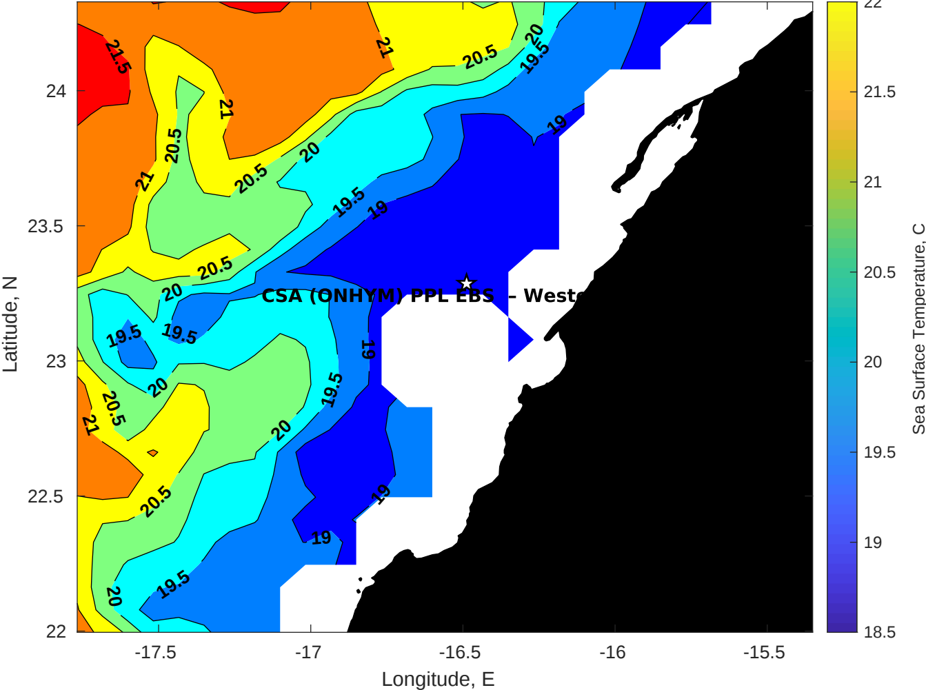
SST for CSA (ONHYM) PPL EBS - Western Sahara at 02-Jan-2026 00:00:00
