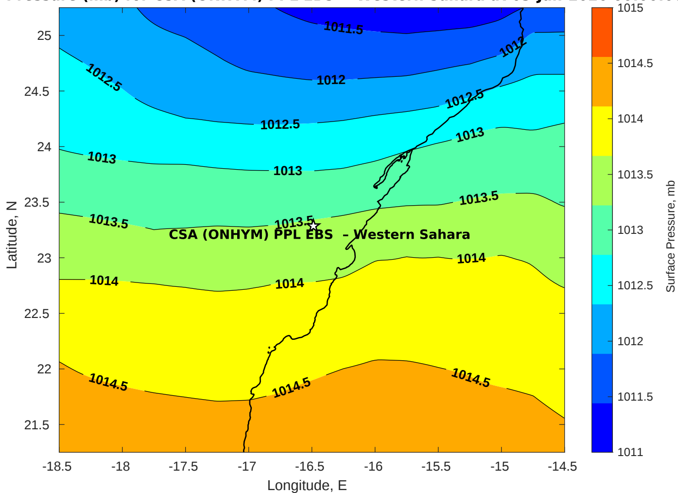
Surface Pressure (mb) for CSA (ONHYM) PPL EBS - Western Sahara at 03-Jan-2026 00:00:00
