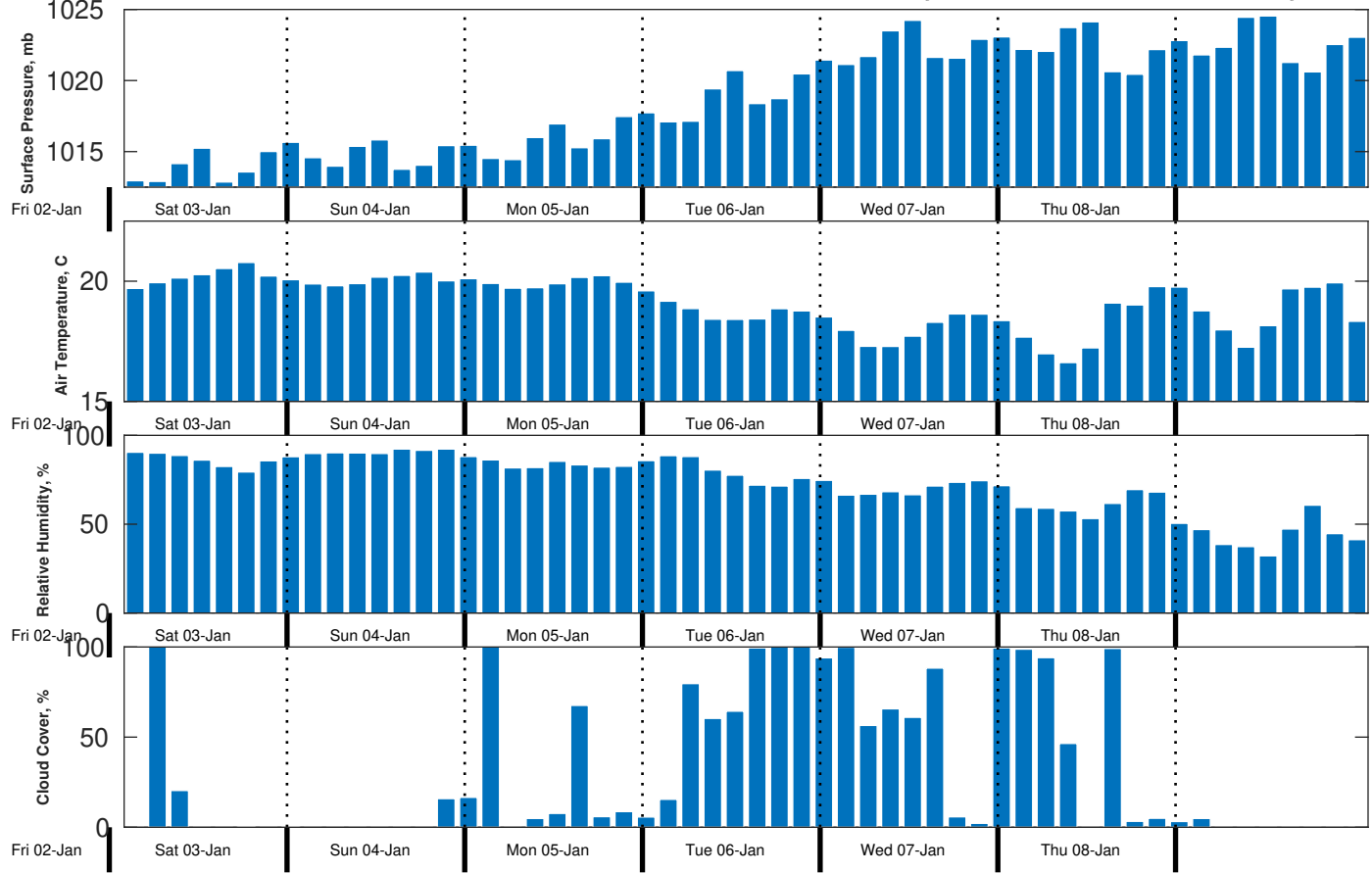
Met Forecast for CSA (ONHYM) PPL EBS - Western Sahara from 03-Jan-2026 00:00:00 to 10-Jan-2026 00:00:00
