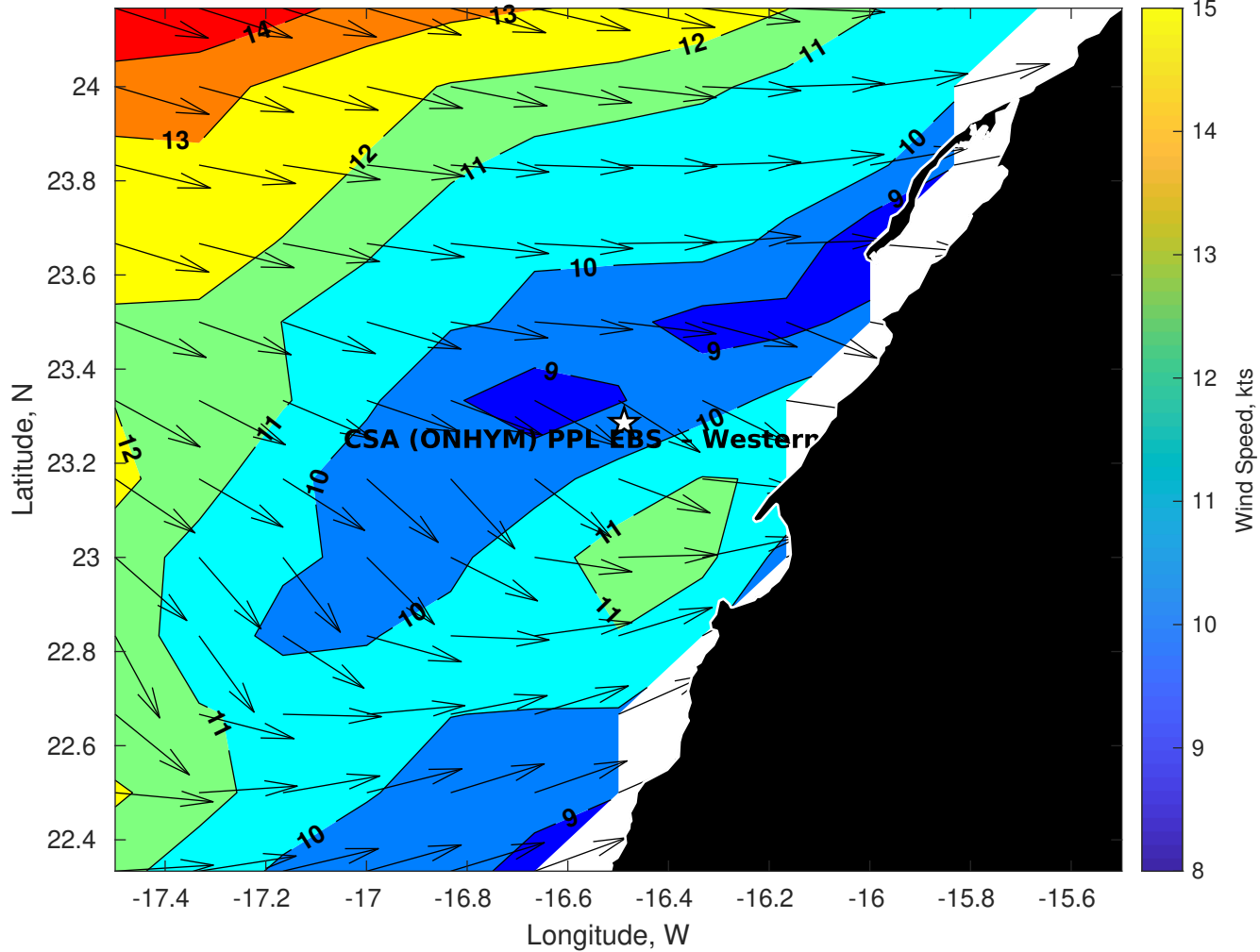
GFS Winds (kts) for CSA (ONHYM) PPL EBS - Western Sahara at 03-Jan-2026 09:00:00
