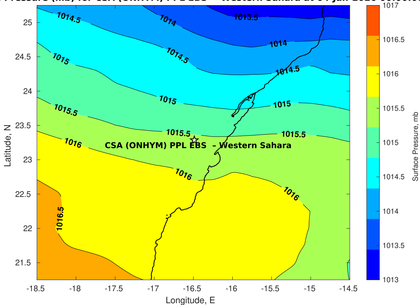
Surface Pressure (mb) for CSA (ONHYM) PPL EBS - Western Sahara at 04-Jan-2026 00:00:00
