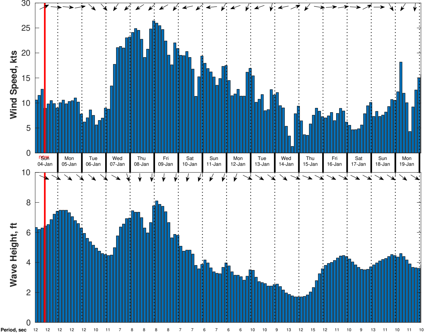
Wind & Wave Forecast for CSA (ONHYM) PPL EBS - Western Sahara from 03-Jan-2026 01:00:00 to 19-Jan-2026 01:00:00
