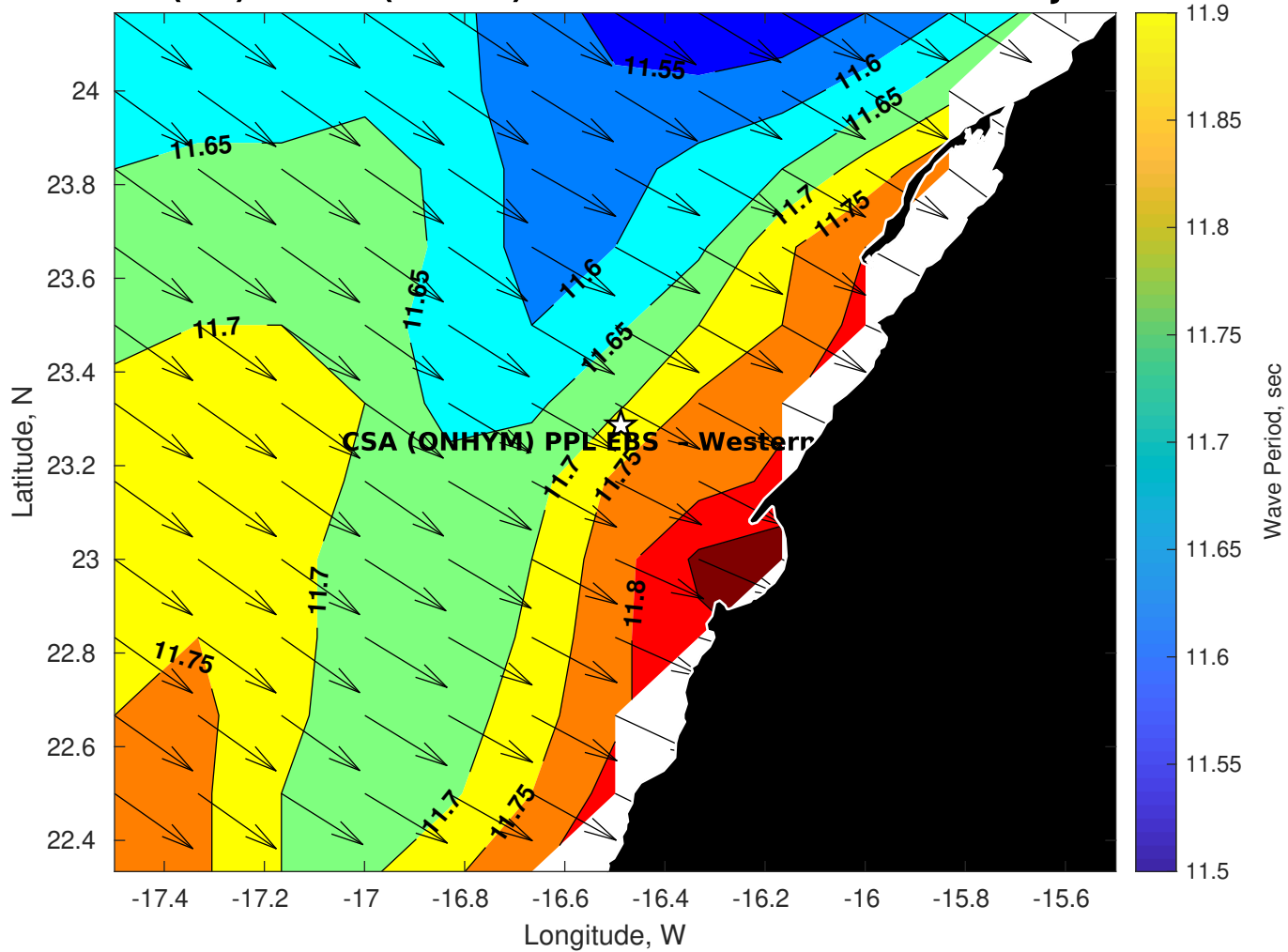
GFS Wave Period (sec) for CSA (ONHYM) PPL EBS - Western Sahara at 03-Jan-2026 09:00:00
