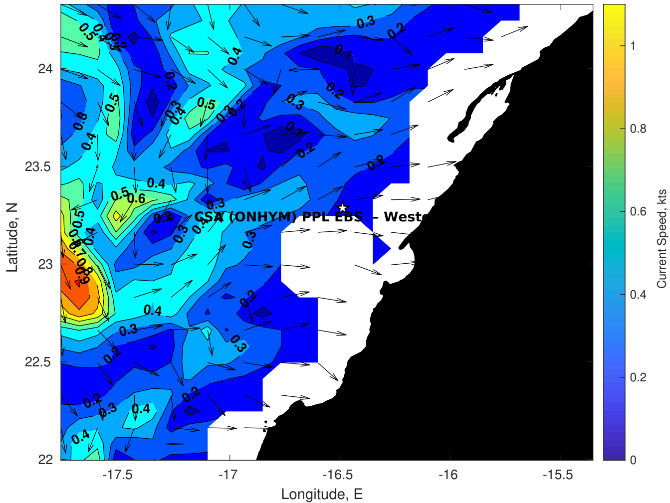
Surface Currents for CSA (ONHYM) PPL EBS - Western Sahara at 02-Jan-2026 00:00:00
