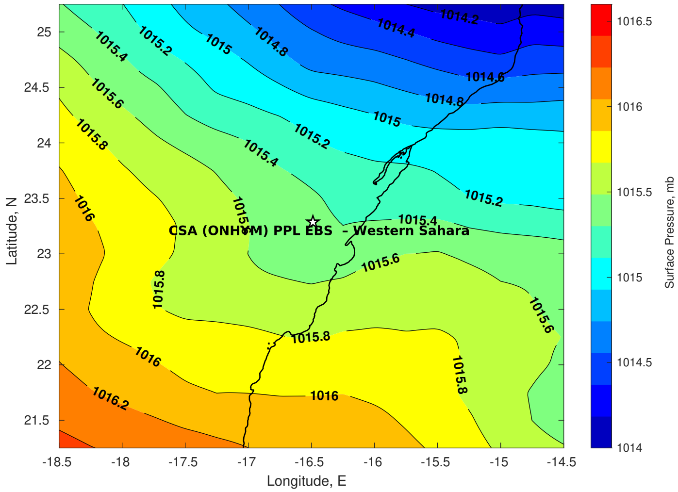
Surface Pressure (mb) for CSA (ONHYM) PPL EBS - Western Sahara at 05-Jan-2026 00:00:00
