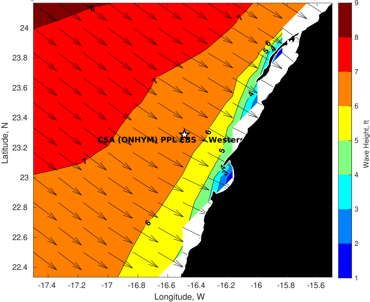
GFS Wave Height (ft) for CSA (ONHYM) PPL EBS - Western Sahara at 03-Jan-2026 09:00:00
