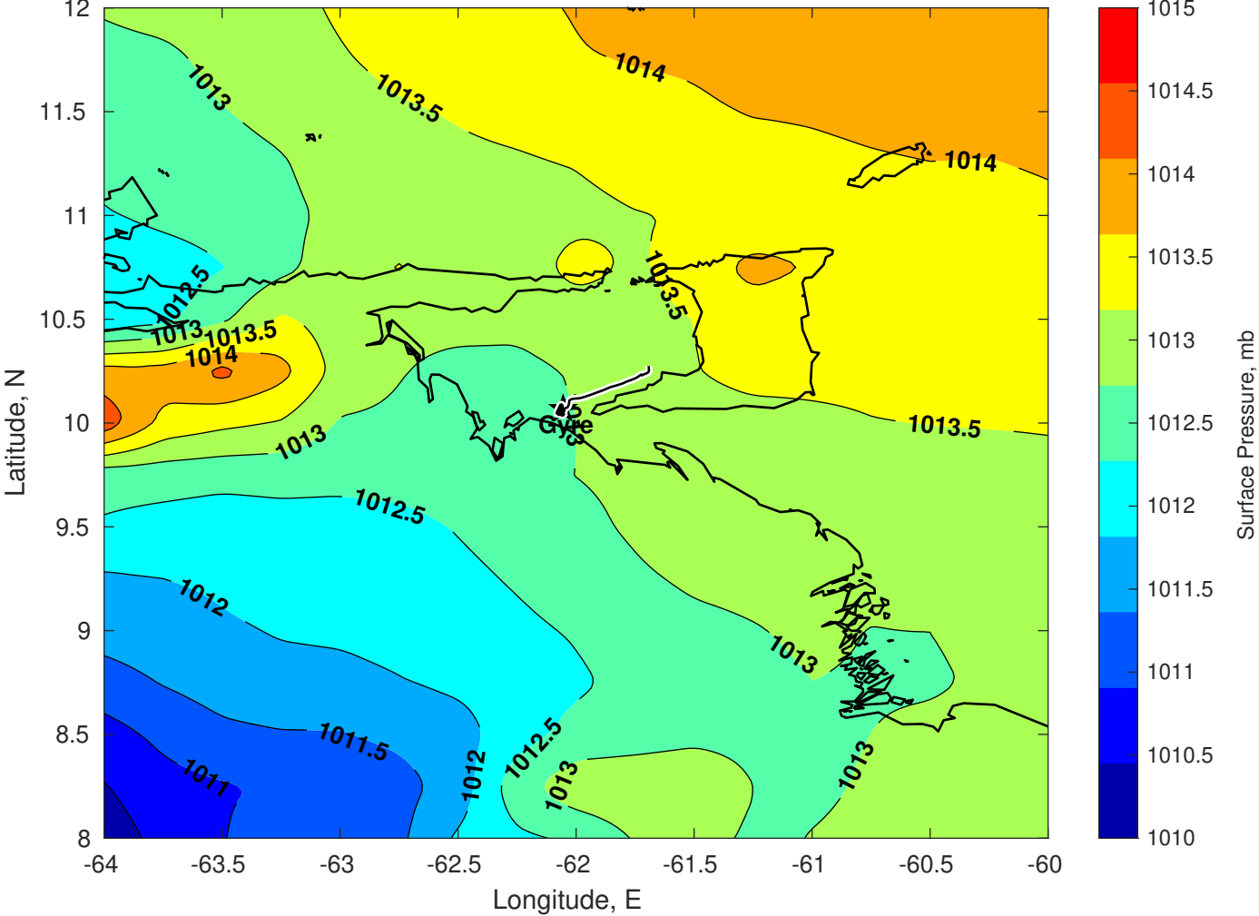
Surface Pressure (mb) for Gyre at 05-Jan-2026 00:00:00
