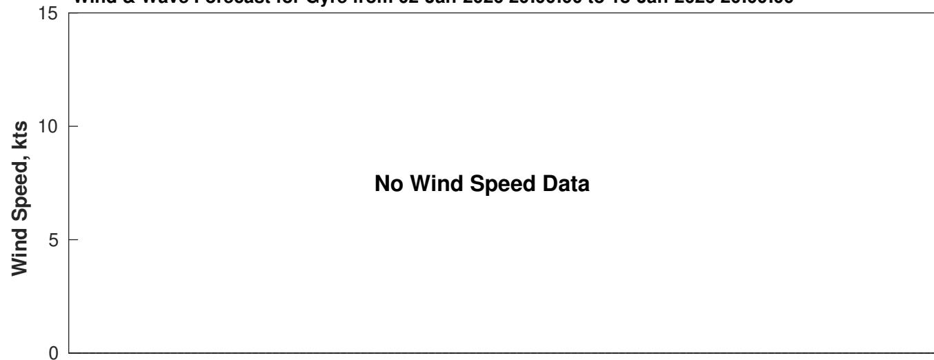
Wind & Wave Forecast for Gyre from 02-Jan-2026 20:00:00 to 18-Jan-2026 20:00:00
