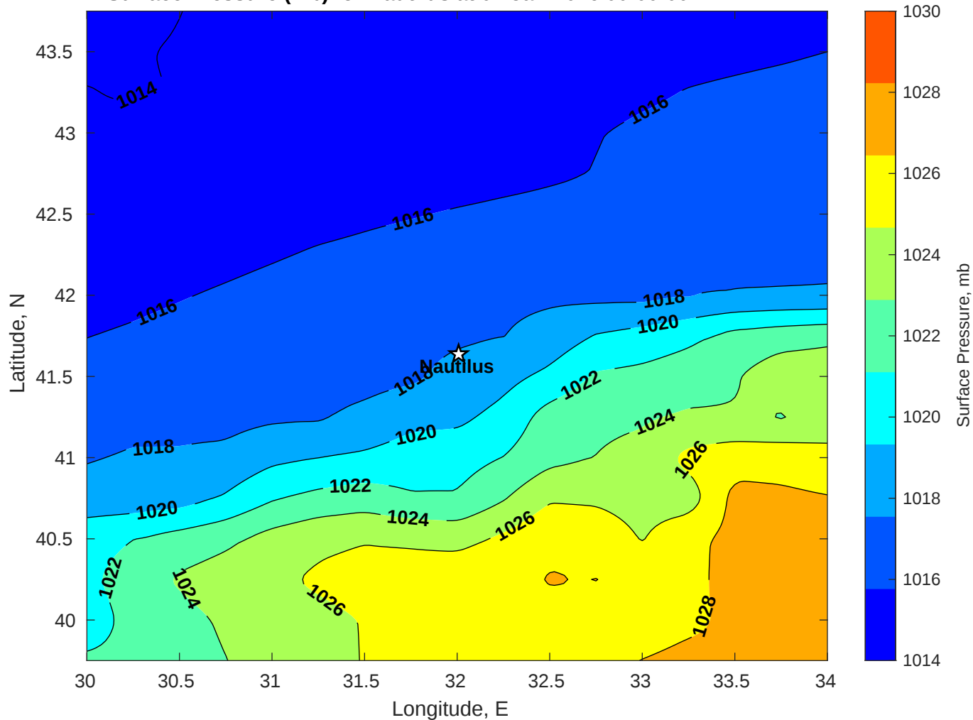
Surface Pressure (mb) for Nautilus at 04-Jan-2026 00:00:00
