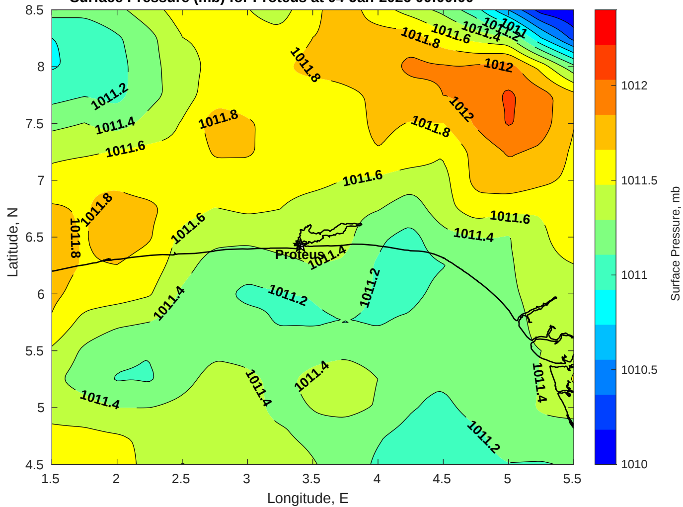
Surface Pressure (mb) for Proteus at 04-Jan-2026 00:00:00
