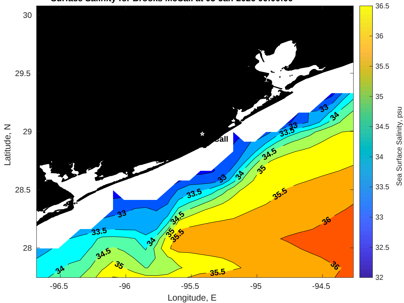
Surface Salinity for Brooks McCall at 03-Jan-2026 00:00:00
