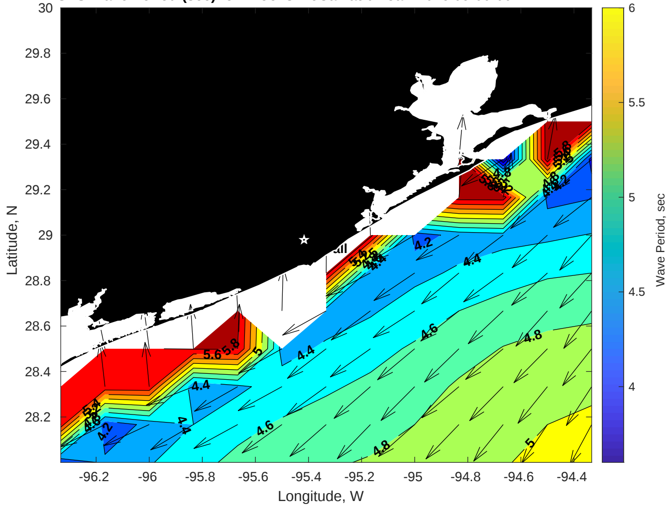
GFS Wave Period (sec) for Brooks McCall at 04-Jan-2026 09:00:00
