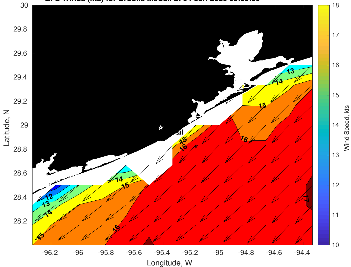
GFS Winds (kts) for Brooks McCall at 04-Jan-2026 09:00:00
