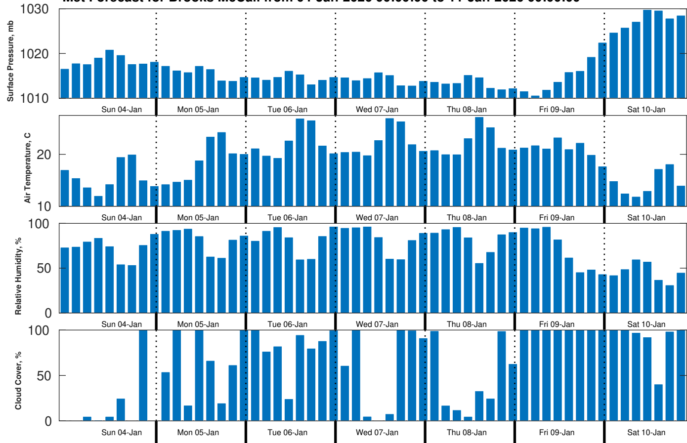
Met Forecast for Brooks McCall from 04-Jan-2026 00:00:00 to 11-Jan-2026 00:00:00
