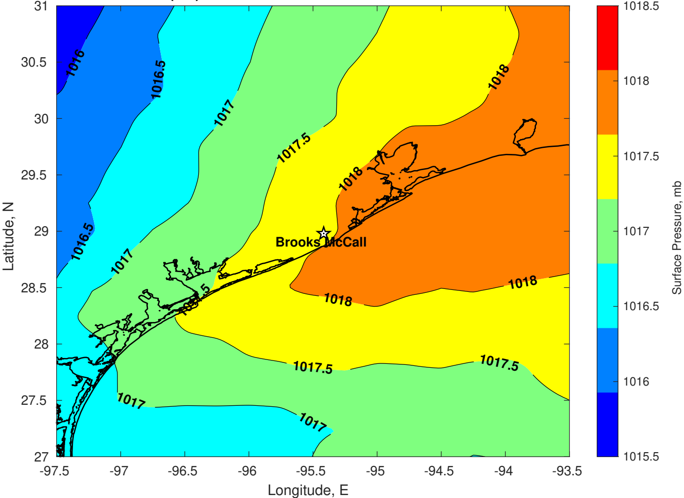
Surface Pressure (mb) for Brooks McCall at 05-Jan-2026 00:00:00
