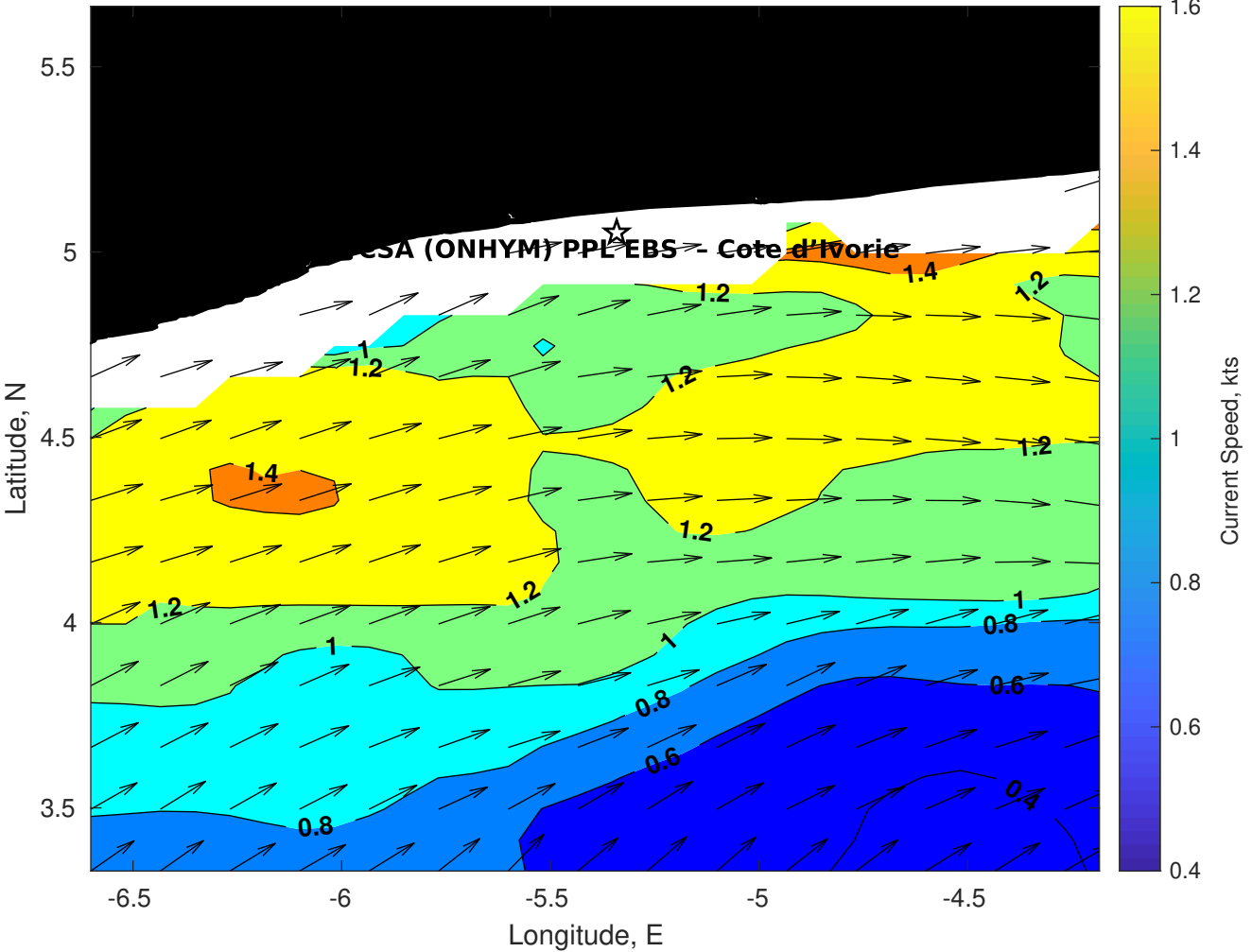
Surface Currents for CSA (ONHYM) PPL EBS - Cote d'Ivoire at 03-Jan-2026 00:00:00
