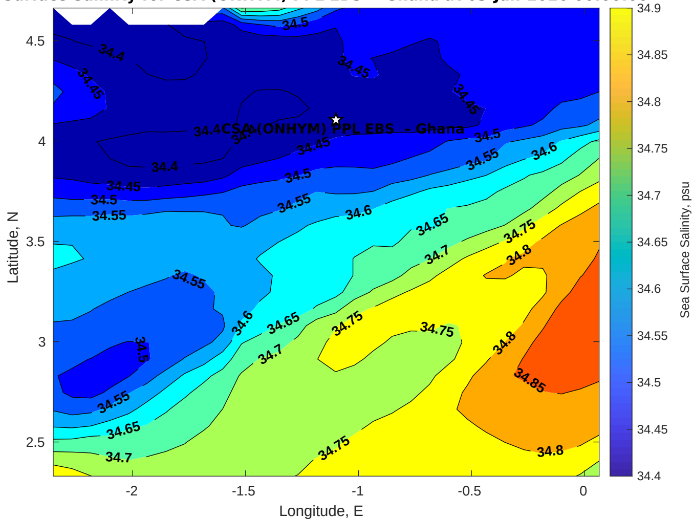
Surface Salinity for CSA (ONHYM) PPL EBS - Ghana at 03-Jan-2026 00:00:00
