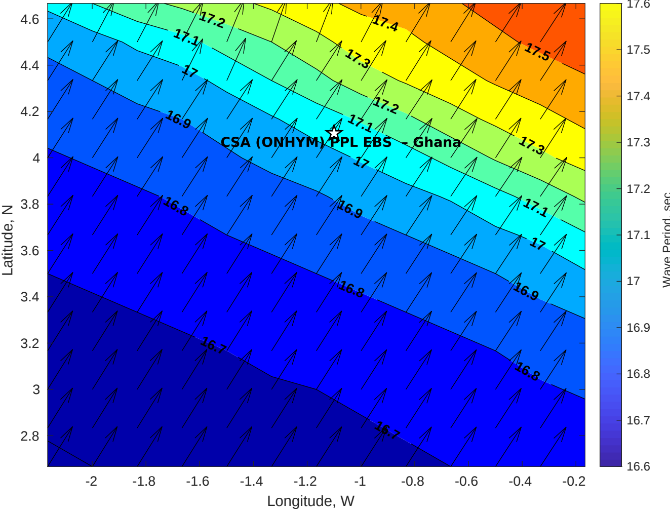
GFS Wave Period (sec) for CSA (ONHYM) PPL EBS - Ghana at 04-Jan-2026 09:00:00
