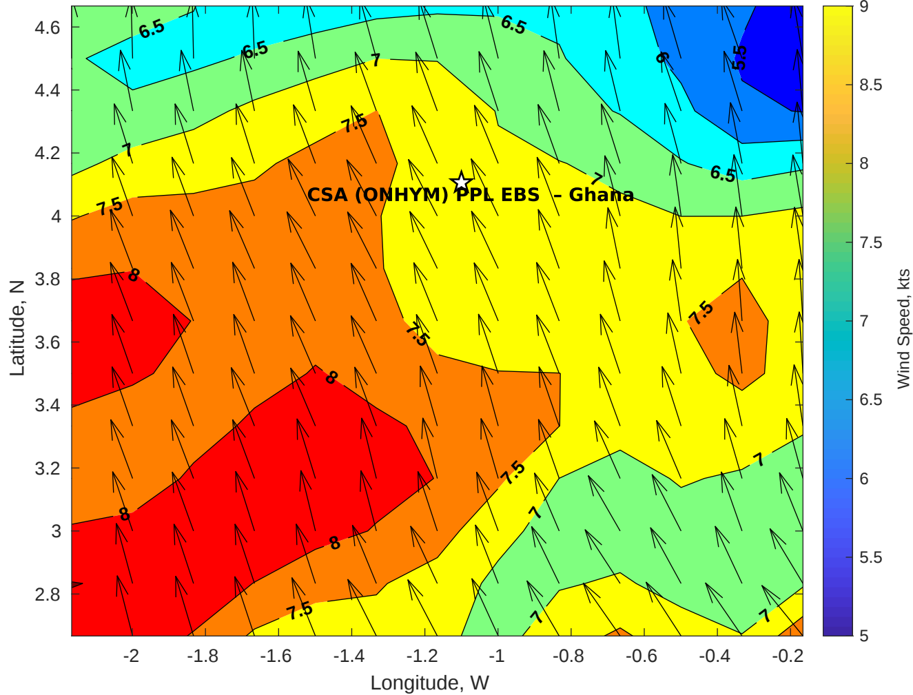
GFS Winds (kts) for CSA (ONHYM) PPL EBS - Ghana at 04-Jan-2026 09:00:00
