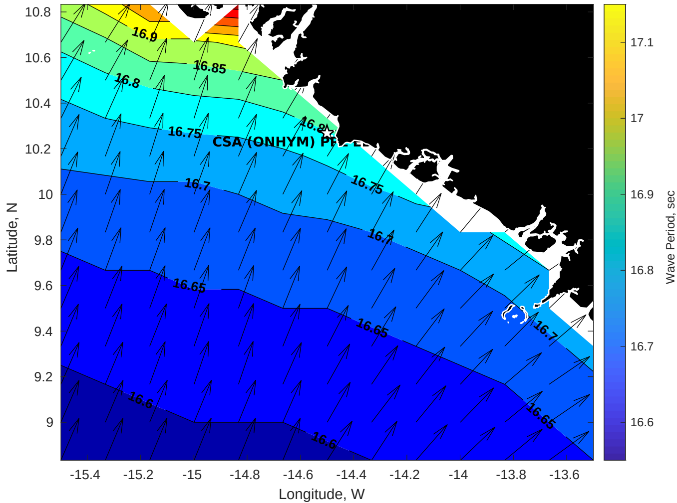
GFS Wave Period (sec) for CSA (ONHYM) PPL EBS - Guinea at 04-Jan-2026 09:00:00
