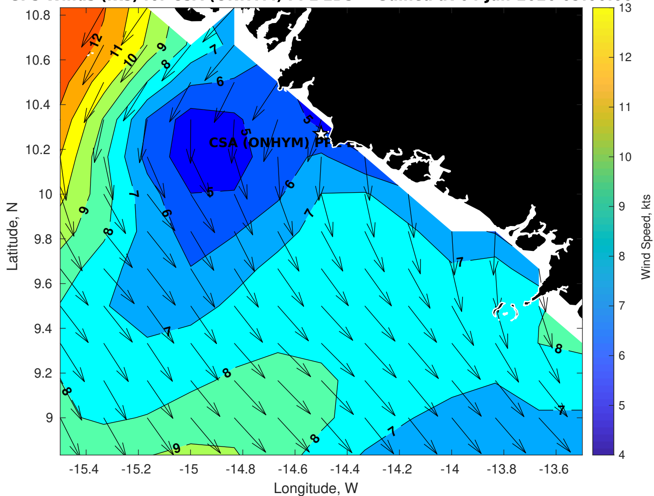
GFS Winds (kts) for CSA (ONHYM) PPL EBS - Guinea at 04-Jan-2026 09:00:00
