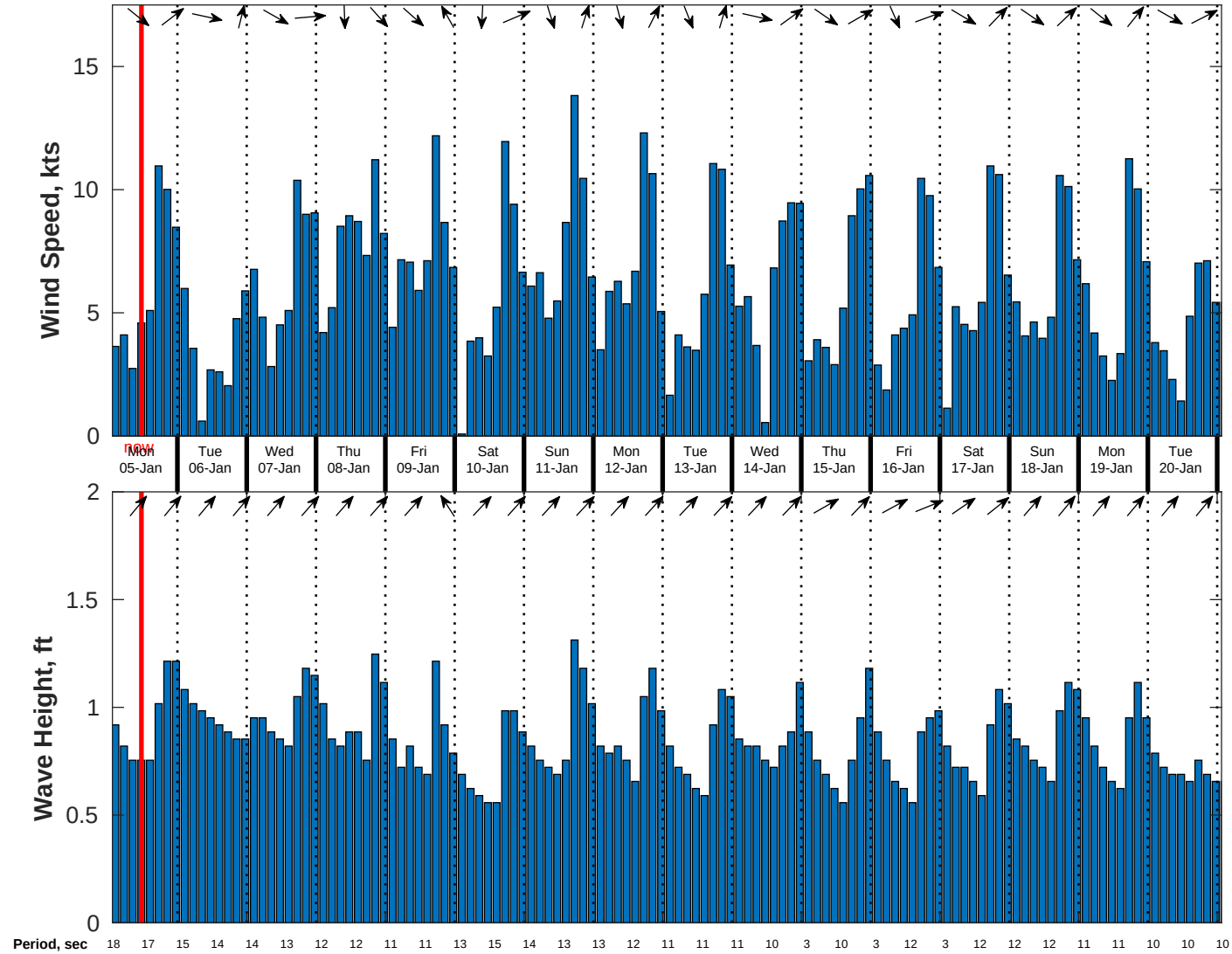
Wind & Wave Forecast for CSA (ONHYM) PPL EBS - Guinea from 04-Jan-2026 01:00:00 to 20-Jan-2026 01:00:00
