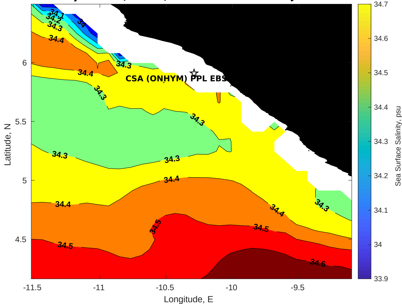
Surface Salinity for CSA (ONHYM) PPL EBS - Liberia at 03-Jan-2026 00:00:00
