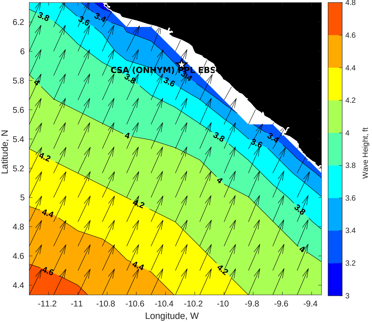
GFS Wave Height (ft) for CSA (ONHYM) PPL EBS - Liberia at 04-Jan-2026 09:00:00
