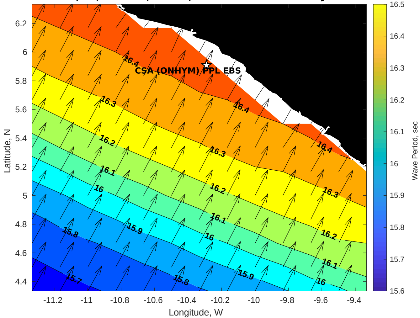
GFS Wave Period (sec) for CSA (ONHYM) PPL EBS - Liberia at 04-Jan-2026 09:00:00
