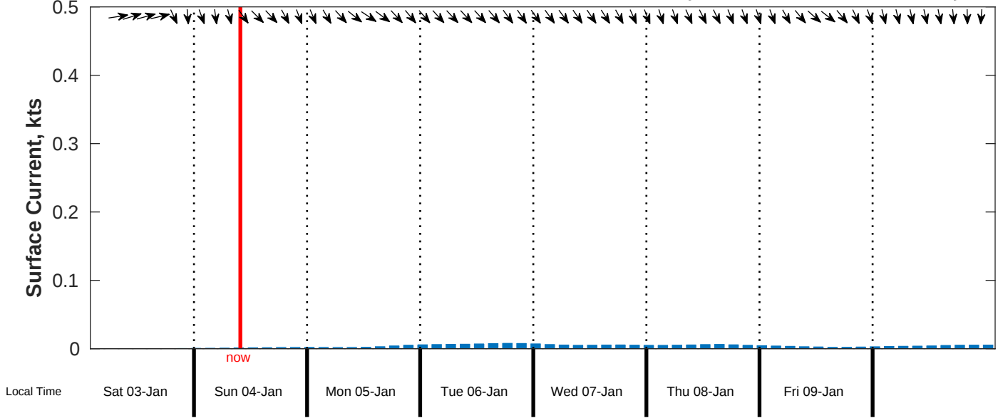
Surface Current Forecast for CSA (ONHYM) PPL EBS - Liberia from 03-Jan-2026 00:00:00 to 11-Jan-2026 00:00:00
