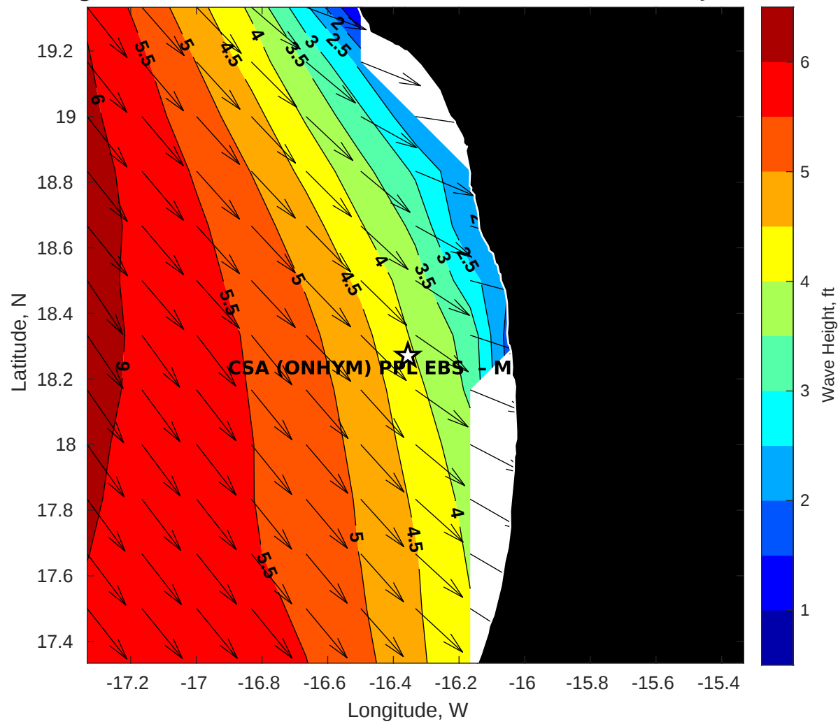
GFS Wave Height (ft) for CSA (ONHYM) PPL EBS - Mauritania at 04-Jan-2026 09:00:00
