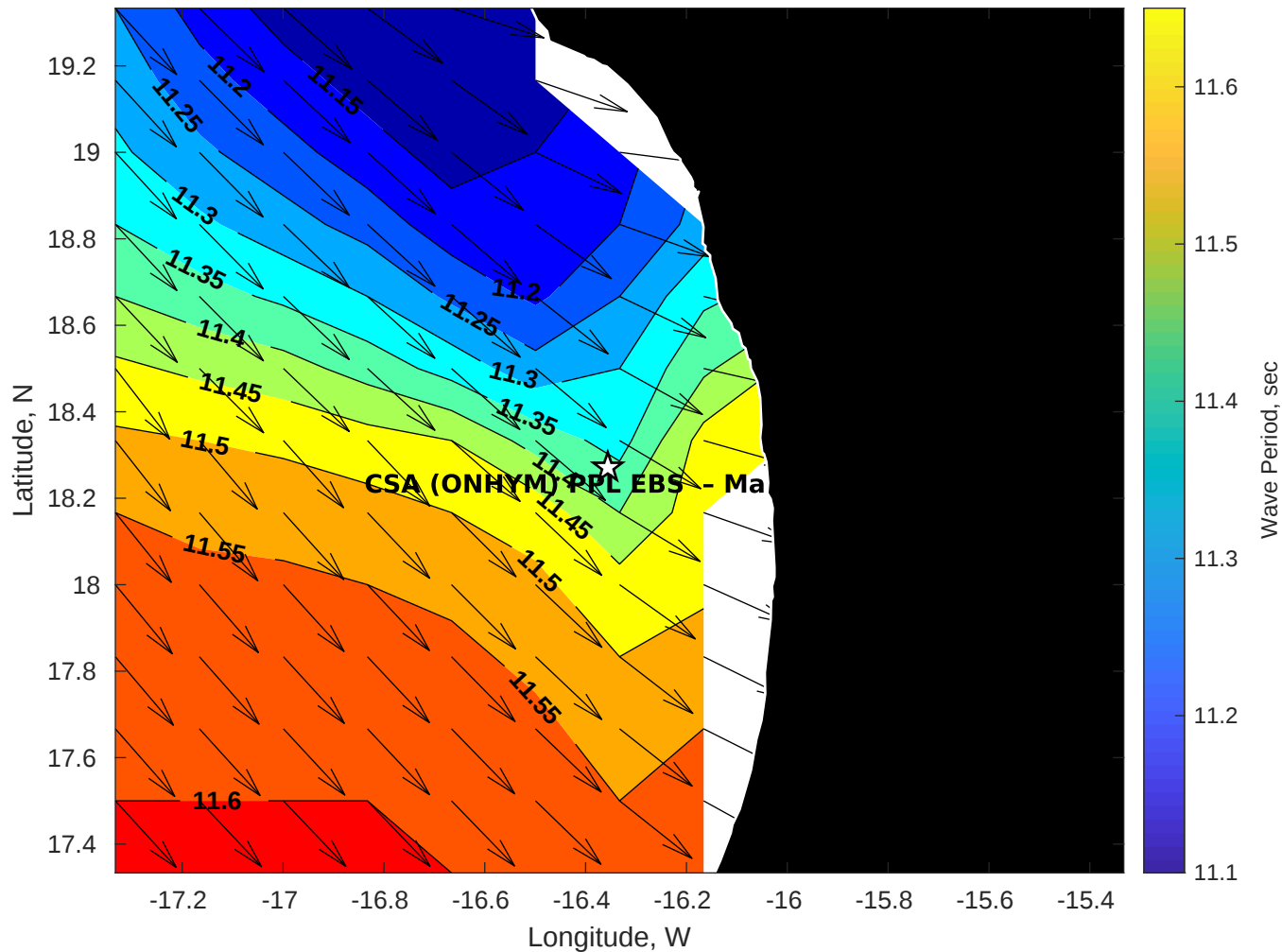
GFS Wave Period (sec) for CSA (ONHYM) PPL EBS - Mauritania at 04-Jan-2026 09:00:00
