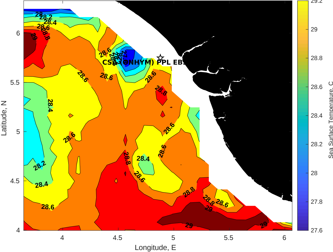
SST for CSA (ONHYM) PPL EBS - Nigeria at 03-Jan-2026 00:00:00
