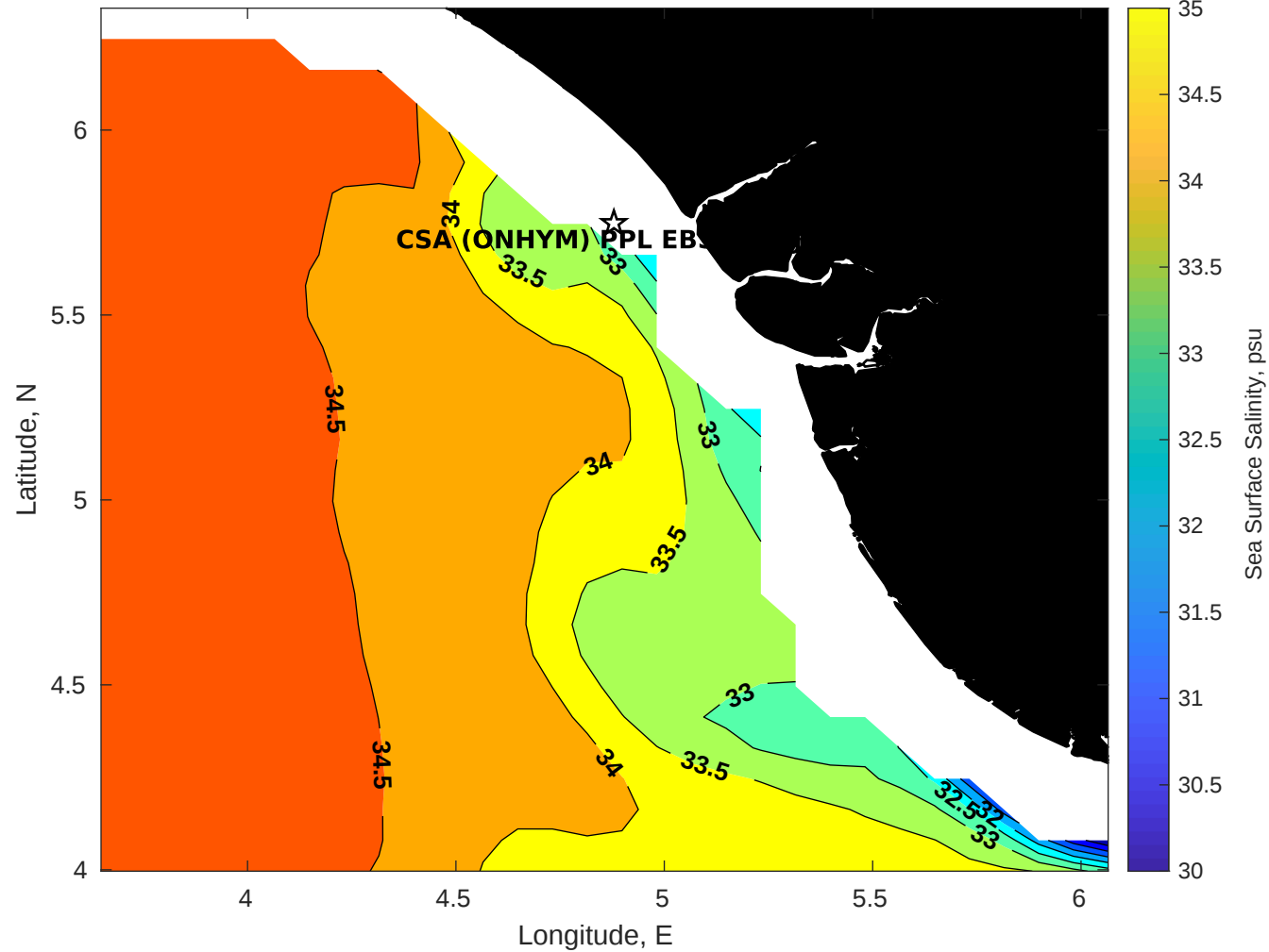
Surface Salinity for CSA (ONHYM) PPL EBS - Nigeria at 03-Jan-2026 00:00:00
