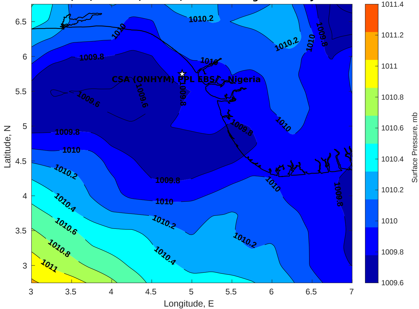
Surface Pressure (mb) for CSA (ONHYM) PPL EBS - Nigeria at 06-Jan-2026 00:00:00
