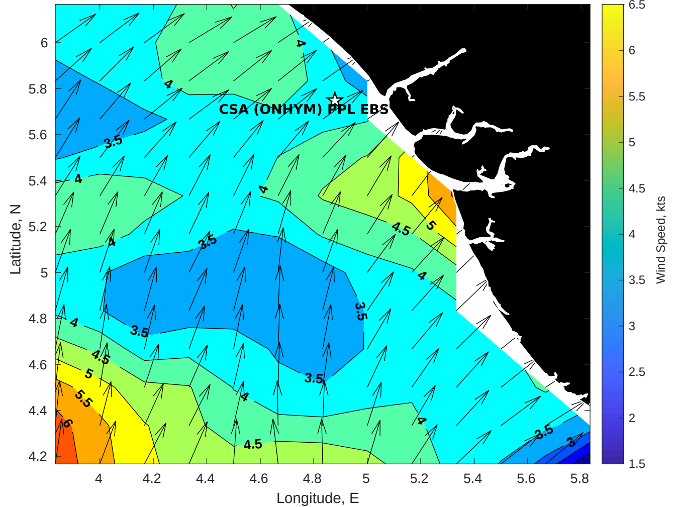
GFS Winds (kts) for CSA (ONHYM) PPL EBS - Nigeria at 04-Jan-2026 09:00:00
