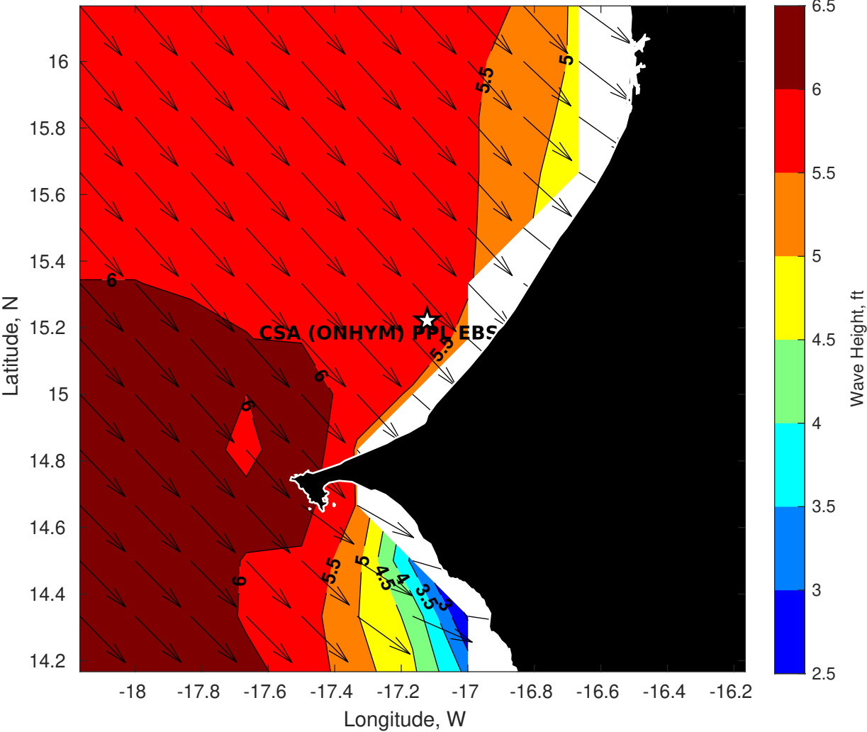
GFS Wave Height (ft) for CSA (ONHYM) PPL EBS - Senegal at 04-Jan-2026 09:00:00
