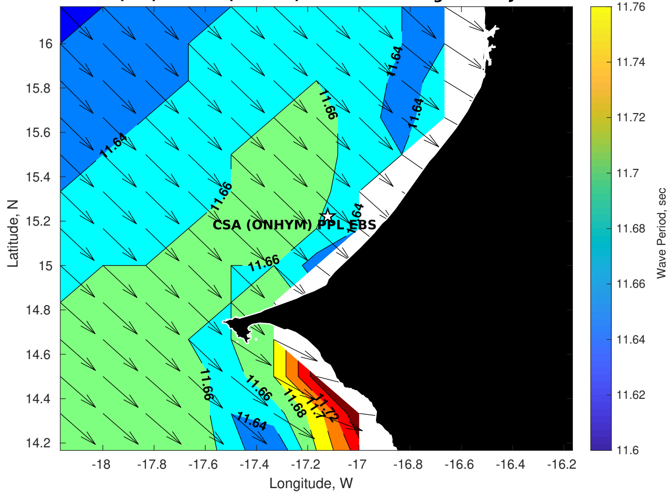
GFS Wave Period (sec) for CSA (ONHYM) PPL EBS - Senegal at 04-Jan-2026 09:00:00
