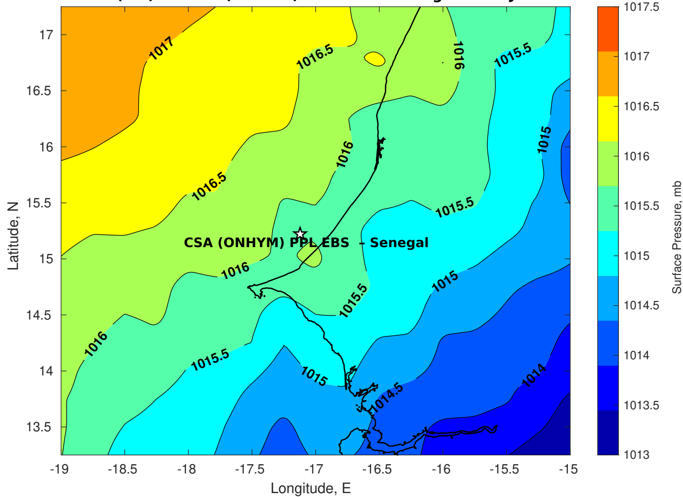
Surface Pressure (mb) for CSA (ONHYM) PPL EBS - Senegal at 05-Jan-2026 00:00:00
