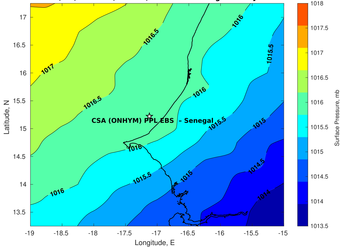
Surface Pressure (mb) for CSA (ONHYM) PPL EBS - Senegal at 06-Jan-2026 00:00:00
