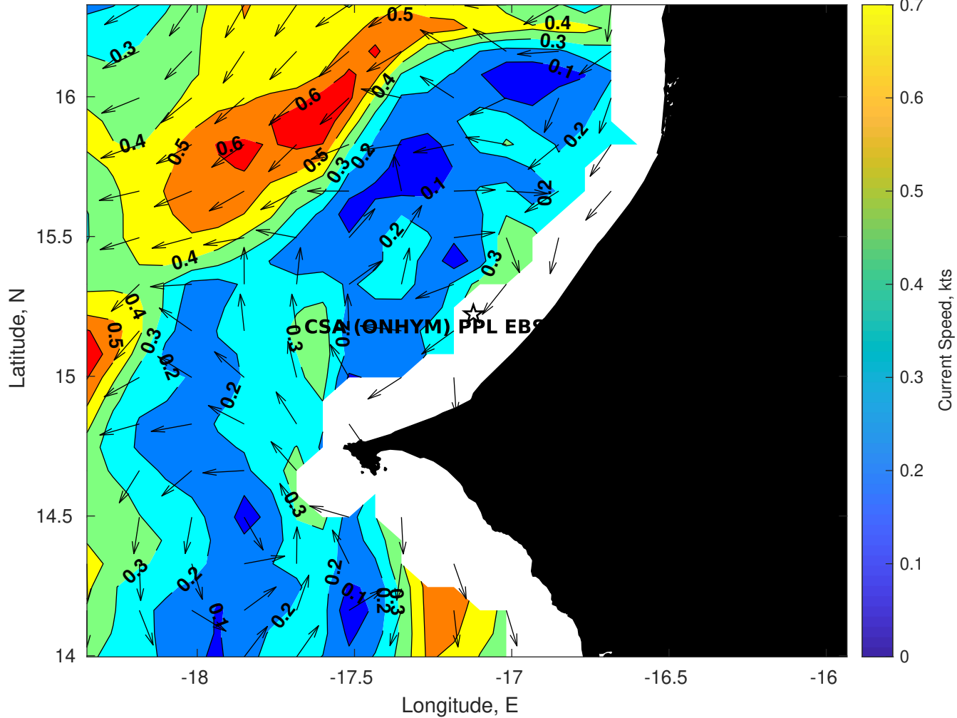
Surface Currents for CSA (ONHYM) PPL EBS - Senegal at 03-Jan-2026 00:00:00
