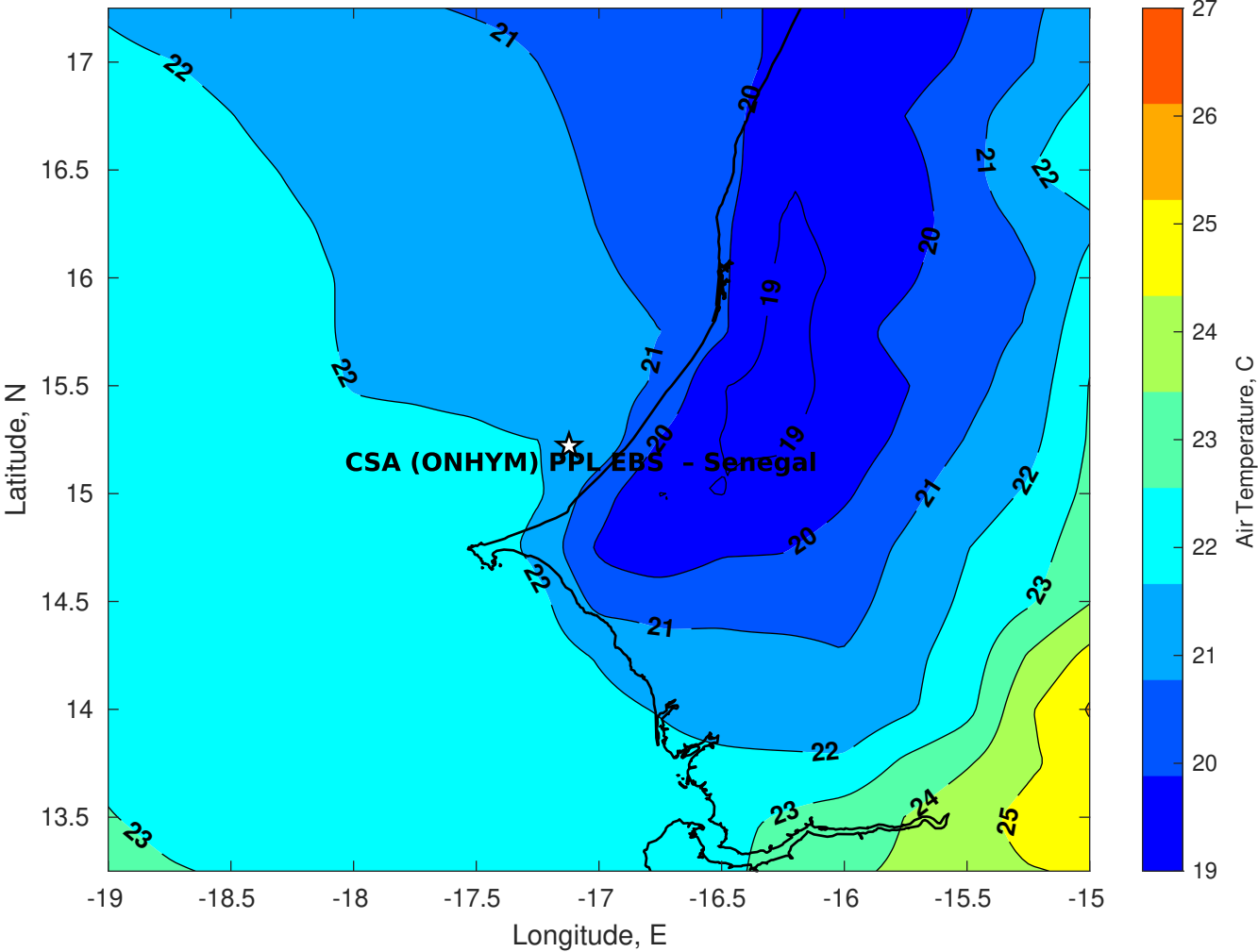
Air Temperature (C) for CSA (ONHYM) PPL EBS - Senegal at 04-Jan-2026
