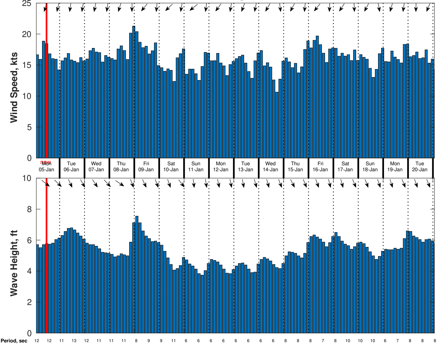
Wind & Wave Forecast for CSA (ONHYM) PPL EBS - Senegal from 04-Jan-2026 01:00:00 to 20-Jan-2026 01:00:00
