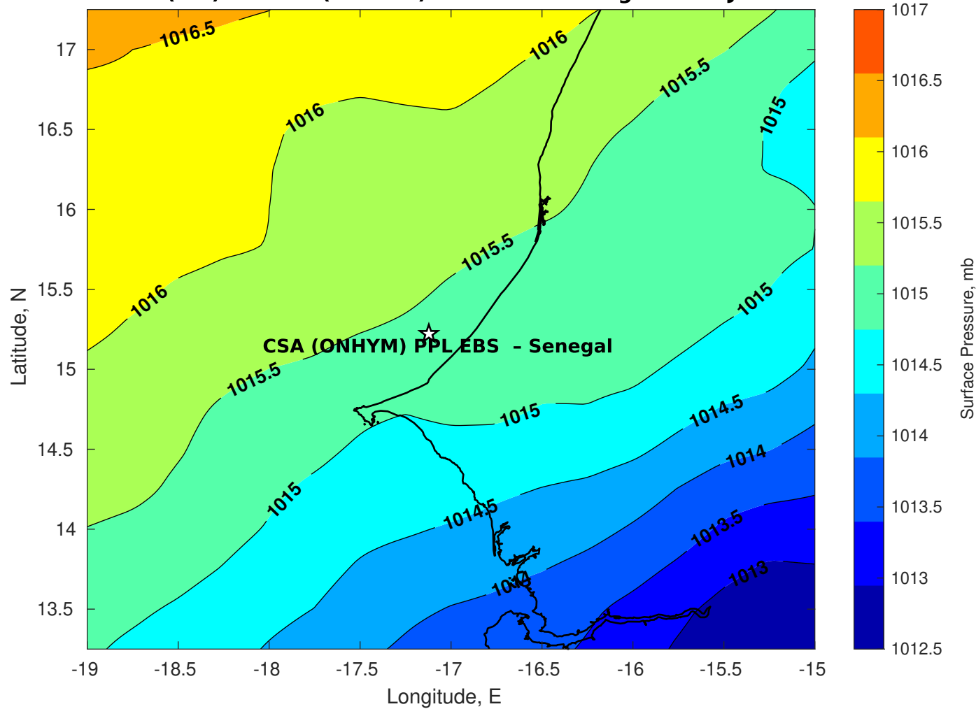
Surface Pressure (mb) for CSA (ONHYM) PPL EBS - Senegal at 04-Jan-2026 00:00:00
