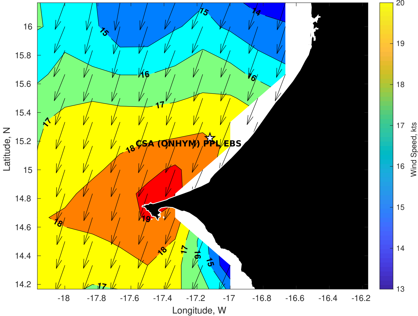
GFS Winds (kts) for CSA (ONHYM) PPL EBS - Senegal at 04-Jan-2026 09:00:00
