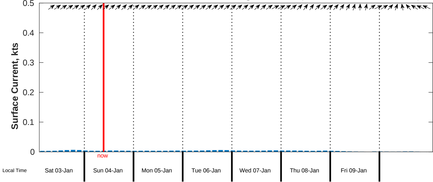
Surface Current Forecast for CSA (ONHYM) PPL EBS - Senegal from 03-Jan-2026 00:00:00 to 11-Jan-2026 00:00:00
