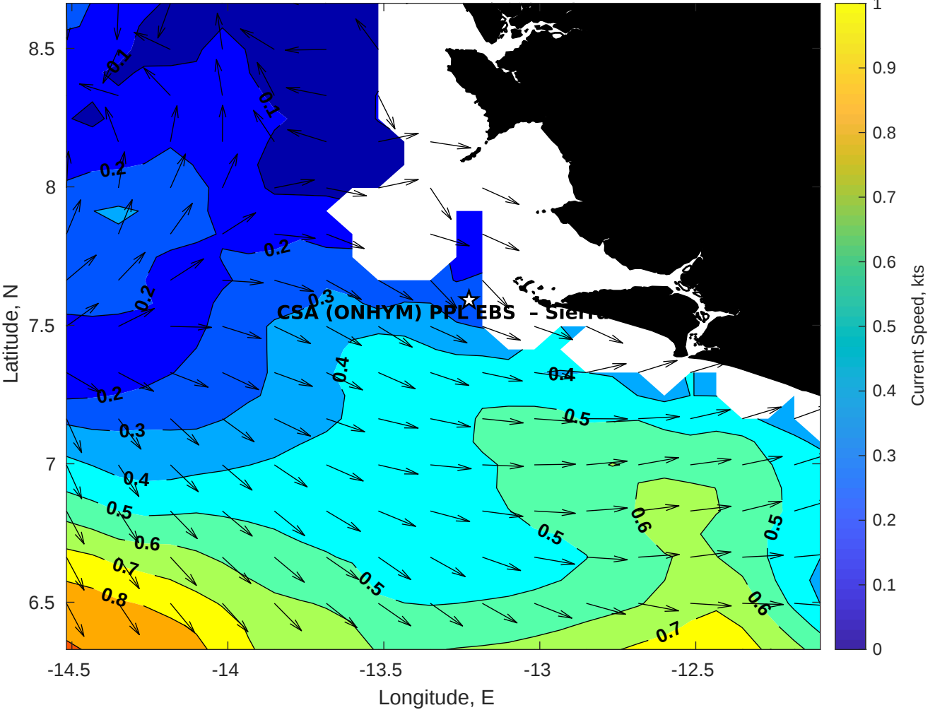
Surface Currents for CSA (ONHYM) PPL EBS - Sierra Leone at 03-Jan-2026 00:00:00
