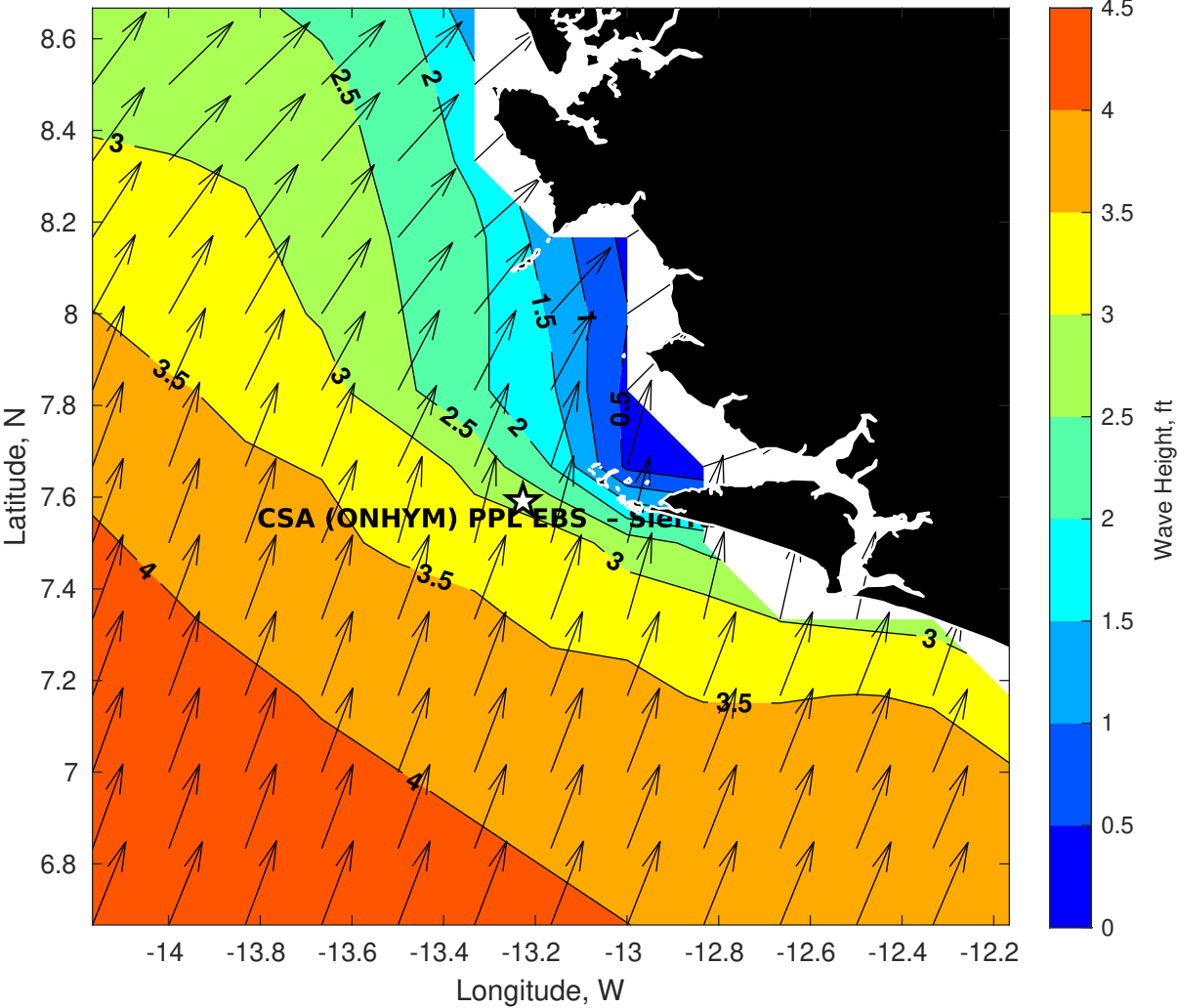
GFS Wave Height (ft) for CSA (ONHYM) PPL EBS - Sierra Leone at 04-Jan-2026 09:00:00
