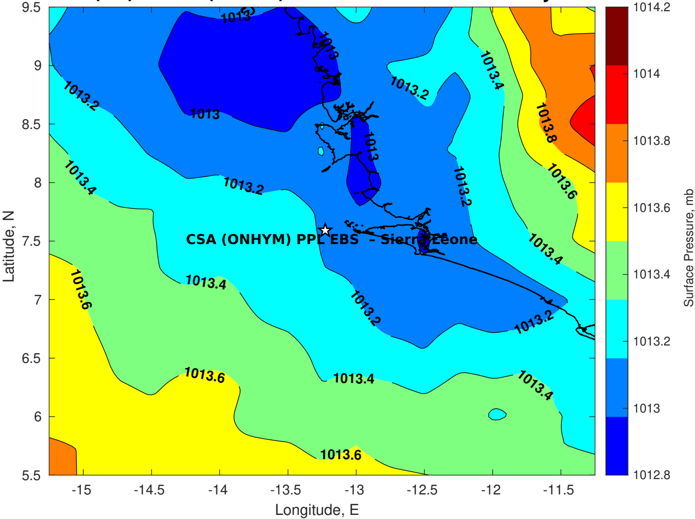
Surface Pressure (mb) for CSA (ONHYM) PPL EBS - Sierra Leone at 06-Jan-2026 00:00:00
