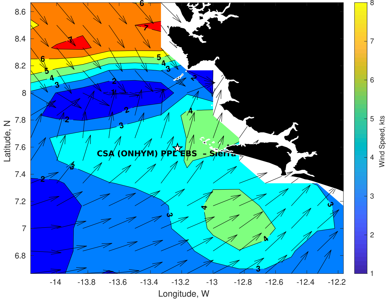
GFS Winds (kts) for CSA (ONHYM) PPL EBS - Sierra Leone at 04-Jan-2026 09:00:00
