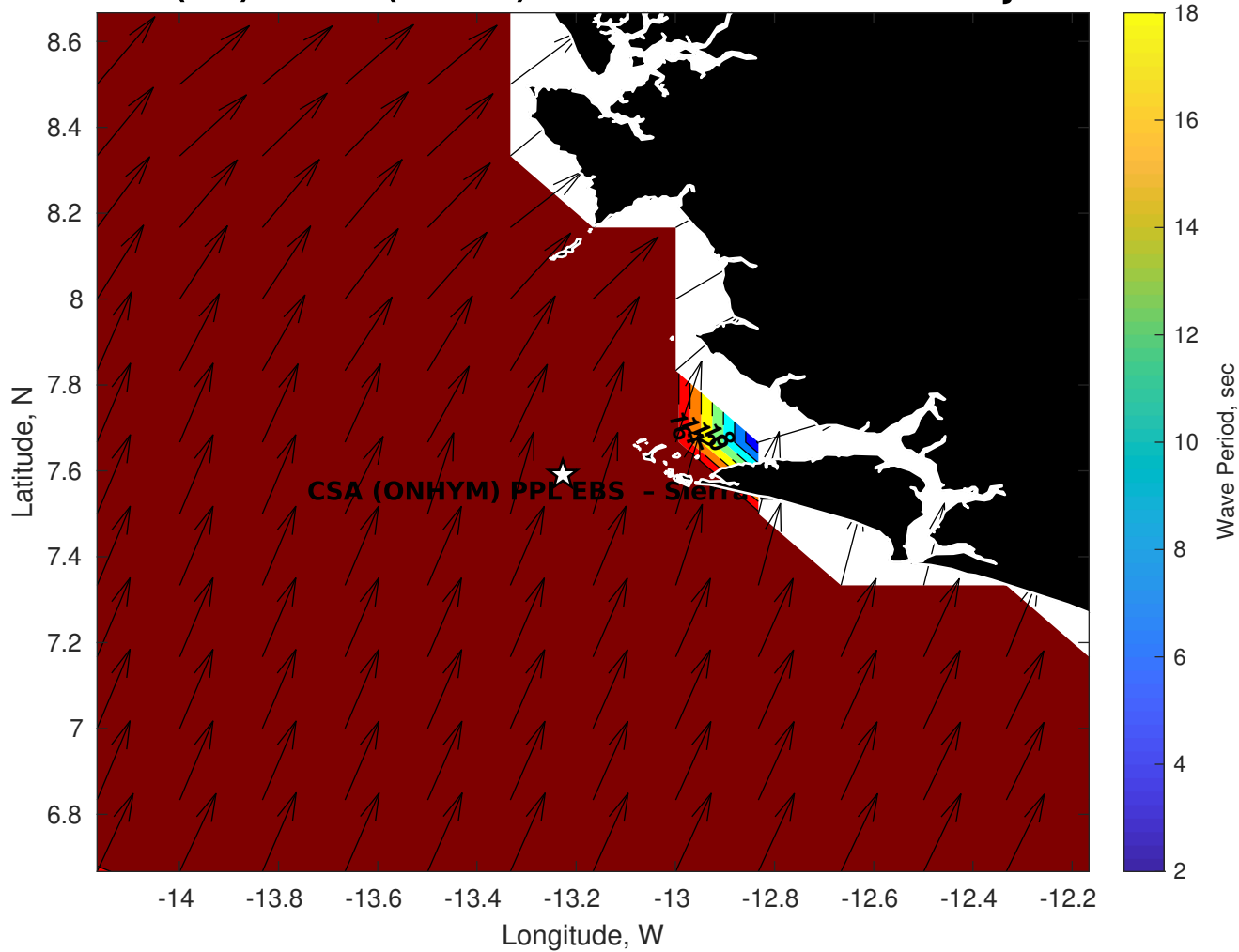
GFS Wave Period (sec) for CSA (ONHYM) PPL EBS - Sierra Leone at 04-Jan-2026 09:00:00
